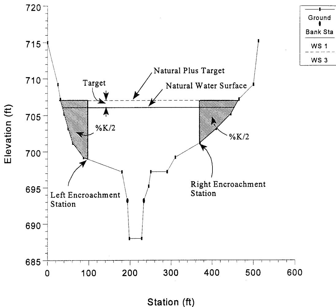
Figure 8.5 Example of Encroachment Method 5
