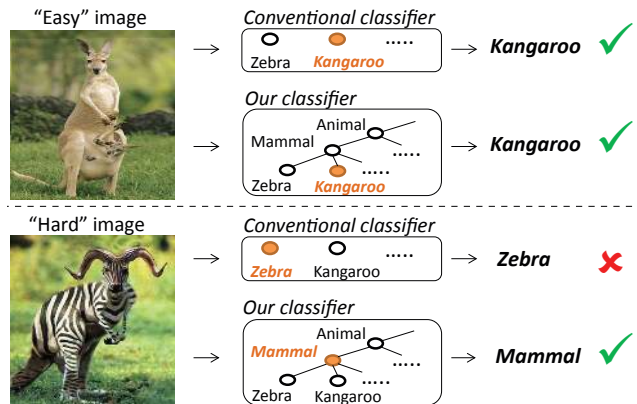
Figure 1. Conventional classifier versus our approach.
