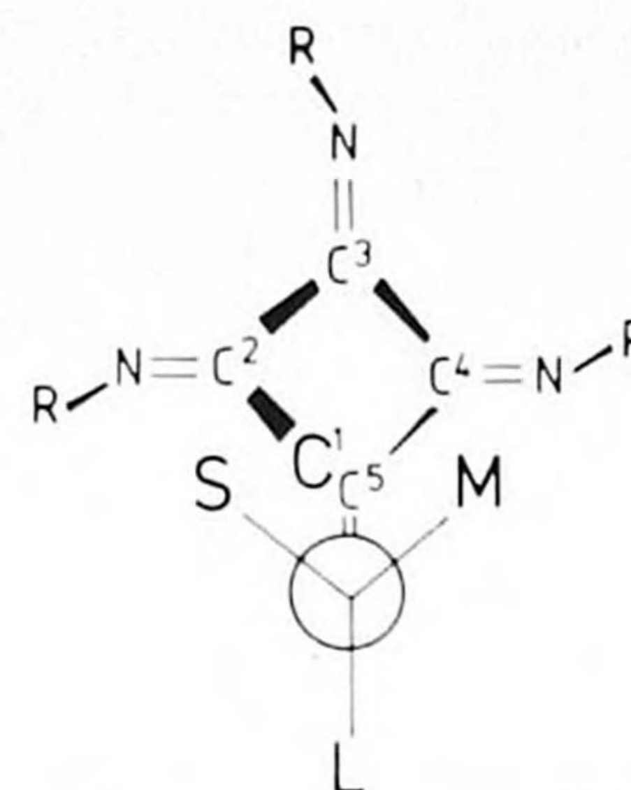
Figure 6. Projection of the side chain (SML)C–N= along the C–N= bond in a P -helical poly(iminomethylene).
