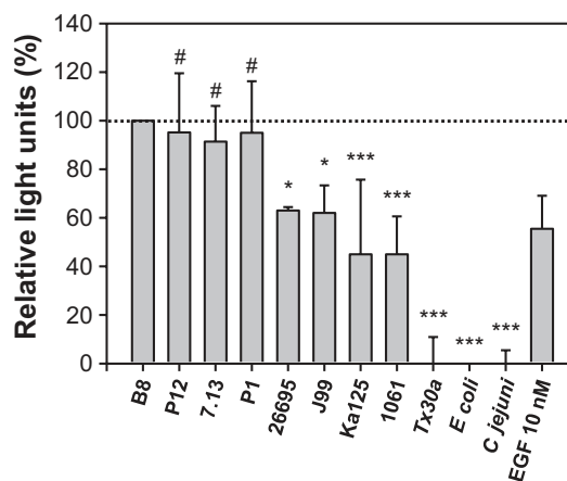
Figure 1 Gastrin promoter activation is H pylori strain specific. AM0 cells were stimulated with H pylori strains, E coli and C jejuni . After infection, cells were harvested and luciferase activity was determined. Luciferase activities in relation to H pylori B8 wild-type (represents 100%; interpolated broken line) were plotted. The mean values \pm SEM of at least three independent experiments are shown. Statistical analysis (Student's t test) was applied using SigmaStat software. *** p \leq 0.001 ; * p \leq 0.05 ; # p > 0.05 . EGF, epidermal growth factor.
