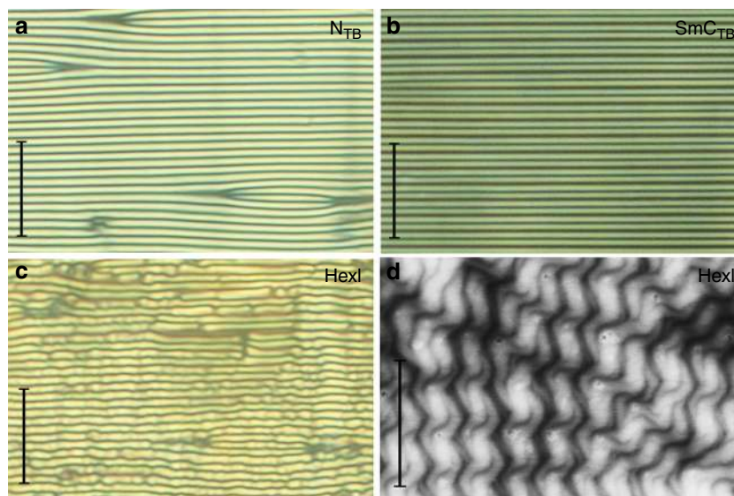
Fig. 3 Optical textures. Stripe textures observed in the 1.9 micron cells with planar anchoring for a N_{TB} phase of CB6OIBeO6, b SmC_{TB} phase of CB6OIBeO7 and c HexI phase of CB6OIBeO6. d AFM image of twisted entangled filaments formed in the temperature range of the HexI phase for homologue CB6OIBeO7. Scale bars in a-c correspond to 20 \mu\text{m} , whereas in d to 500 nm
