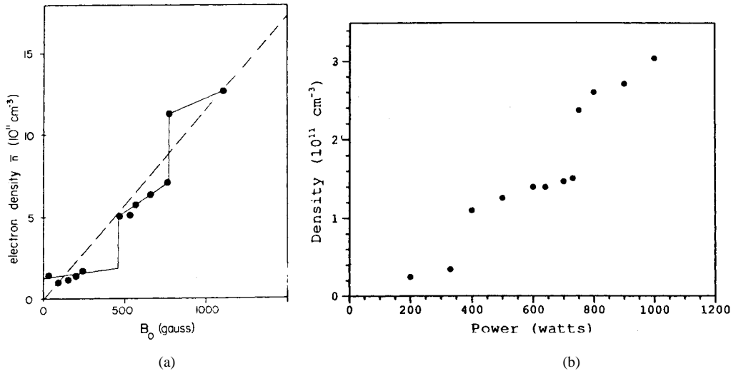
Fig. 7. (a) Density jumps as B_0 is increased (from [5]) and (b) density jump as P_{rf} is increased [115].
