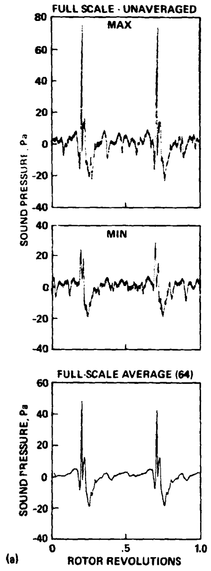
Figure 7.- Comparison of unaveraged and averaged sound pressure time-histories for one rotor revolution. (a) Full-scale (540) rotor; (b) model-scale OLS rotor.
