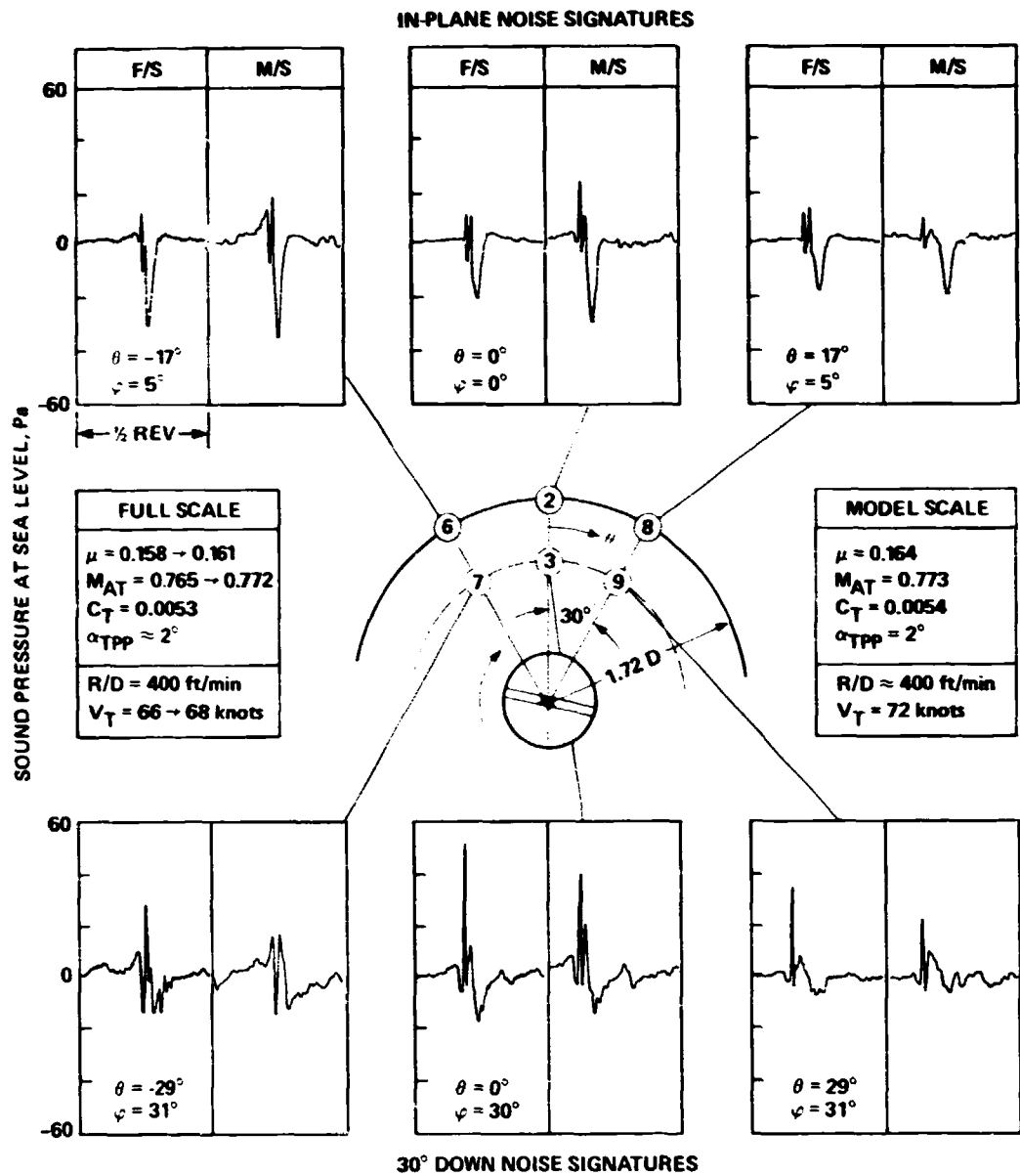
(b) Lateral directivity.
