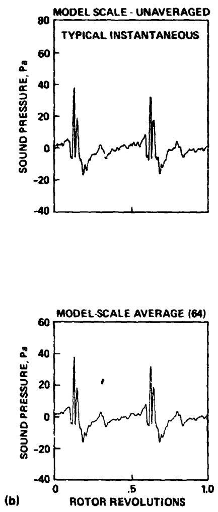
Figure 7.- Comparison of unaveraged and averaged sound pressure time-histories for one rotor revolution. (a) Full-scale (540) rotor; (b) model-scale OLS rotor.
