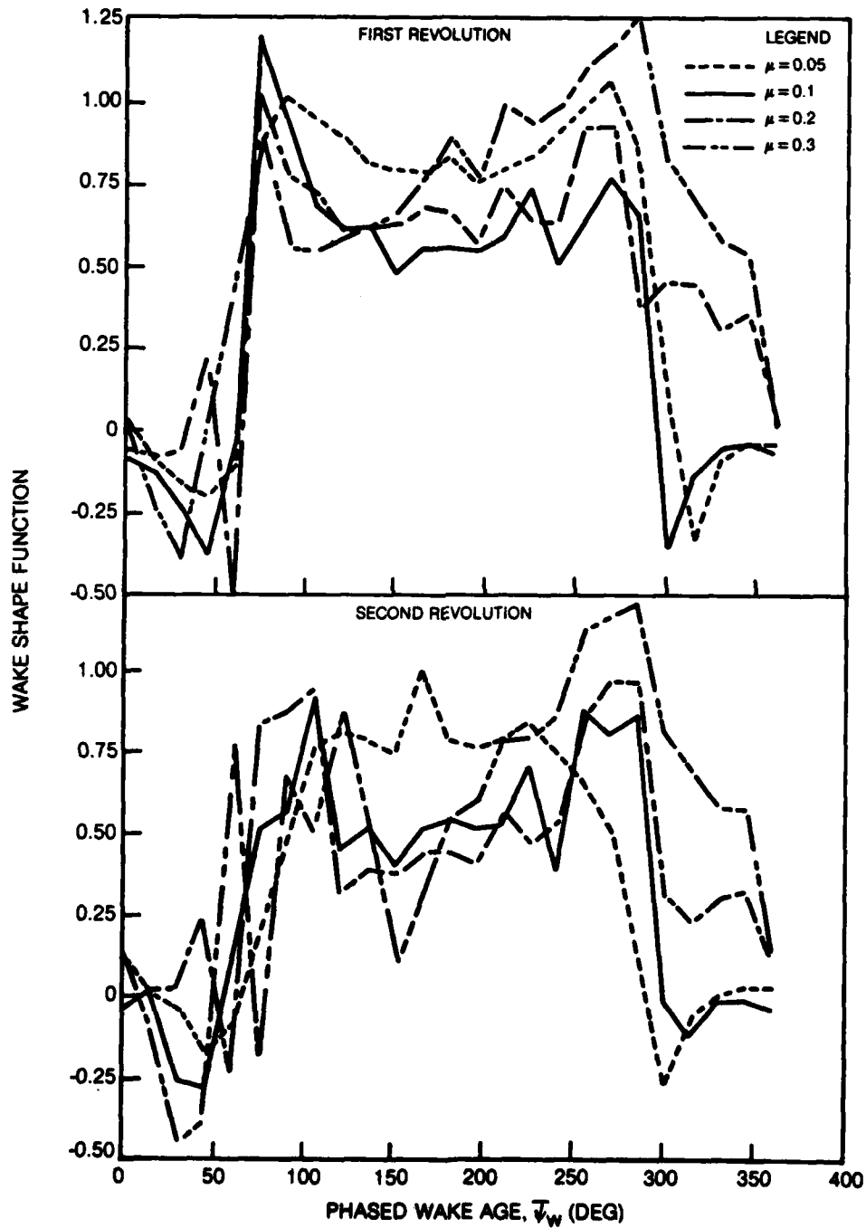
Figure 32. Variation of the Generalized Wake Shape Function with Advance Ratio for the Two-Bladed Representative Rotor
