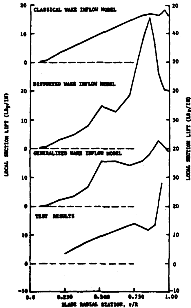
FIGURE 97. COMPARISON OF PREDICTED SPANWISE LOADING FOR H-34 ROTOR AT AN ADVANCE RATIO OF .120, \psi = 90^\circ
