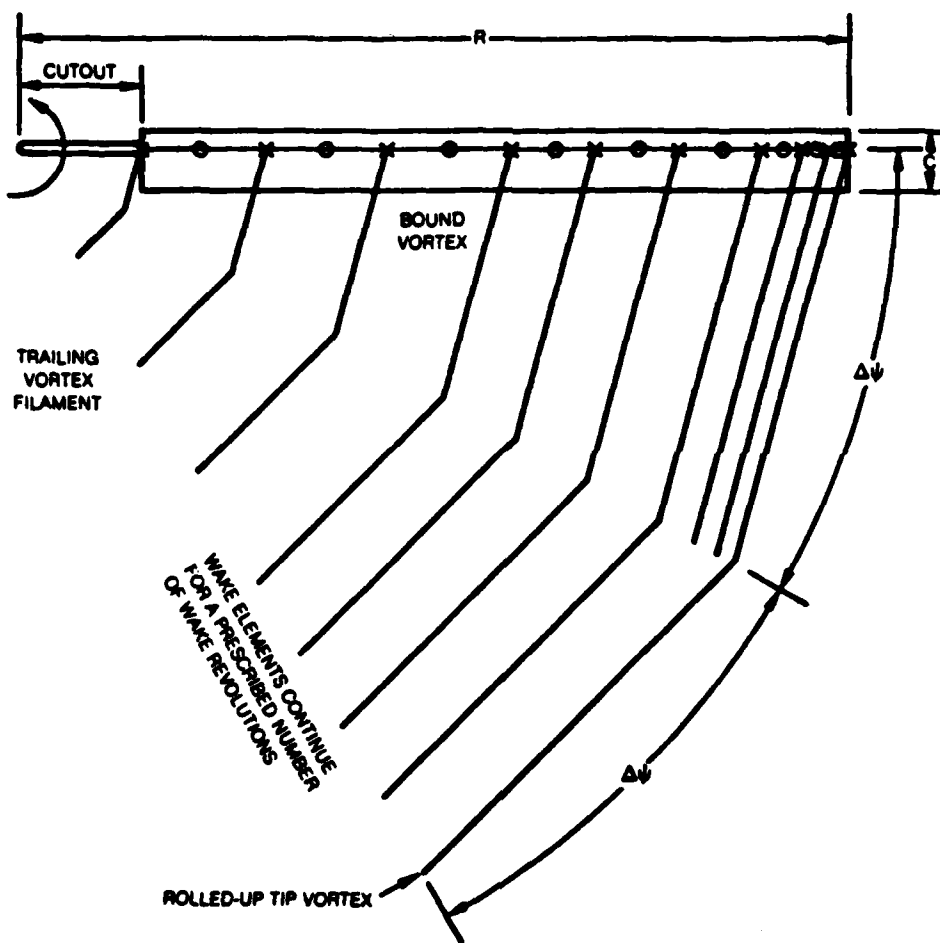
FIGURE 11. REPRESENTATION OF BLADE AND WAKE BY BOUND AND TRAILING VORTEX SEGMENTS
