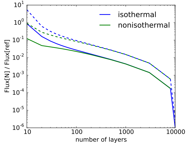
Figure 2. Mean (solid curves) and maximum (dashed curves) errors in the synthetic spectrum as a function of the number of model layers used, computed by performing retrievals on the measured spectrum of HR 8799b. The reference used is the retrieval with 10,000 model layers (see text). When about 100 layers are used, the models with isothermal and non-isothermal layers yield the same answers.
