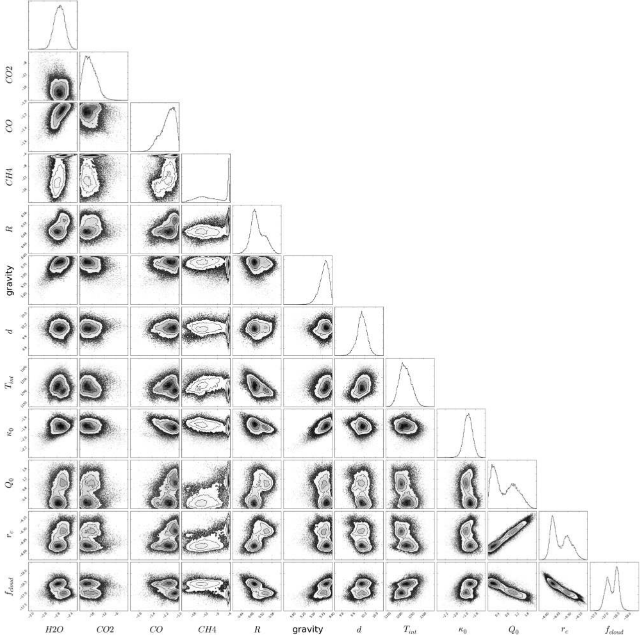
Figure 6. Montage of posterior distributions from performing retrieval on the measured spectrum of HR 8799b and allowing the radius, surface gravity and mean molecular weights to be uniform or log-uniform priors. The retrieved value of the radius ( R \approx 0.5R_J ) is unphysical (see text for discussion). The labels “CO”, “CO 2 ”, “CH 4 ” and “H 2 O” refer to the mixing ratios of carbon monoxide, carbon dioxide, methane and water, respectively. R and T_{\text{int}} are in units of R_J and K, respectively. The labels “ \kappa_0 ” and “gravity” are for \log \kappa_0 and \log g in mks and cgs units, respectively.
