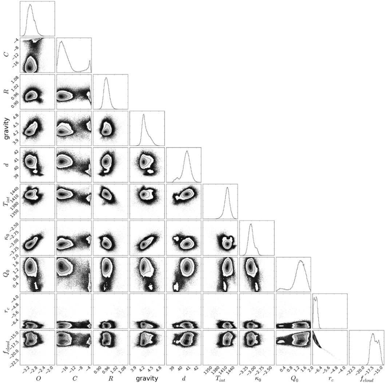
Figure B4. Same as Figure B2, but for HR 8799d.
