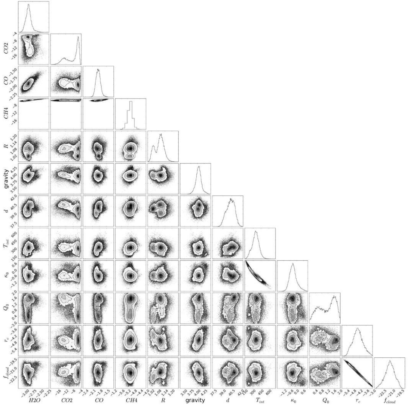
Figure B2. Montage of posterior distributions from the best-fit retrieval model of HR 8799b.
