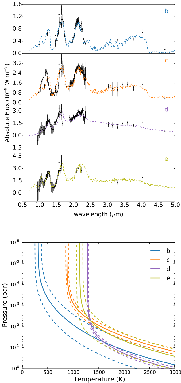
Figure 9. Best-fit spectra and temperature-pressure profiles for HR 8799b, c, d and e.
