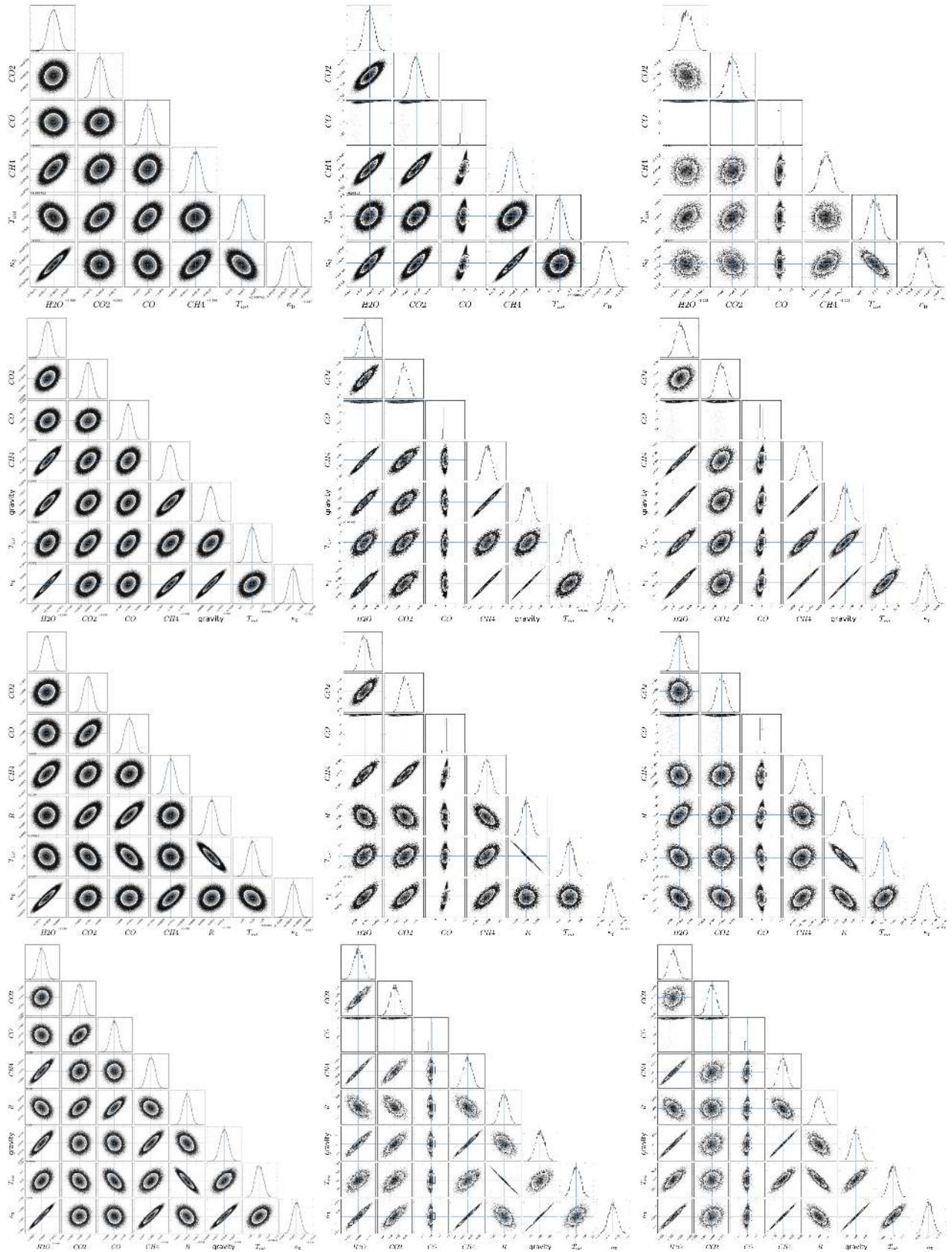
Figure 4. Performing retrieval on a mock dataset, where the “ground truth” is known (see text for input parameters). We focus on performing retrieval with the UB model (see Table 1). The columns represent the different wavelength coverages: 0.7\text{--}5\ \mu\text{m} with 0.01\ \mu\text{m} resolution (first column), HR 8799b-like data (second column) and HR 8799e-like data (third column). The rows represent different assumptions for R and g : fixed R and g (first row), fixed R but g is a fitting parameter (second row), fixed g but R is a fitting parameter (third row), both R and g are fitting parameters (fourth row). The labels “CO”, “CO 2 ”, “CH 4 ” and “H 2 O” refer to the mixing ratios of carbon monoxide, carbon dioxide, methane and water, respectively. T_{\text{int}} is in units of K. The labels “ \kappa_0 ” and “gravity” are for \log \kappa_0 and \log g in mks and cgs units, respectively.
