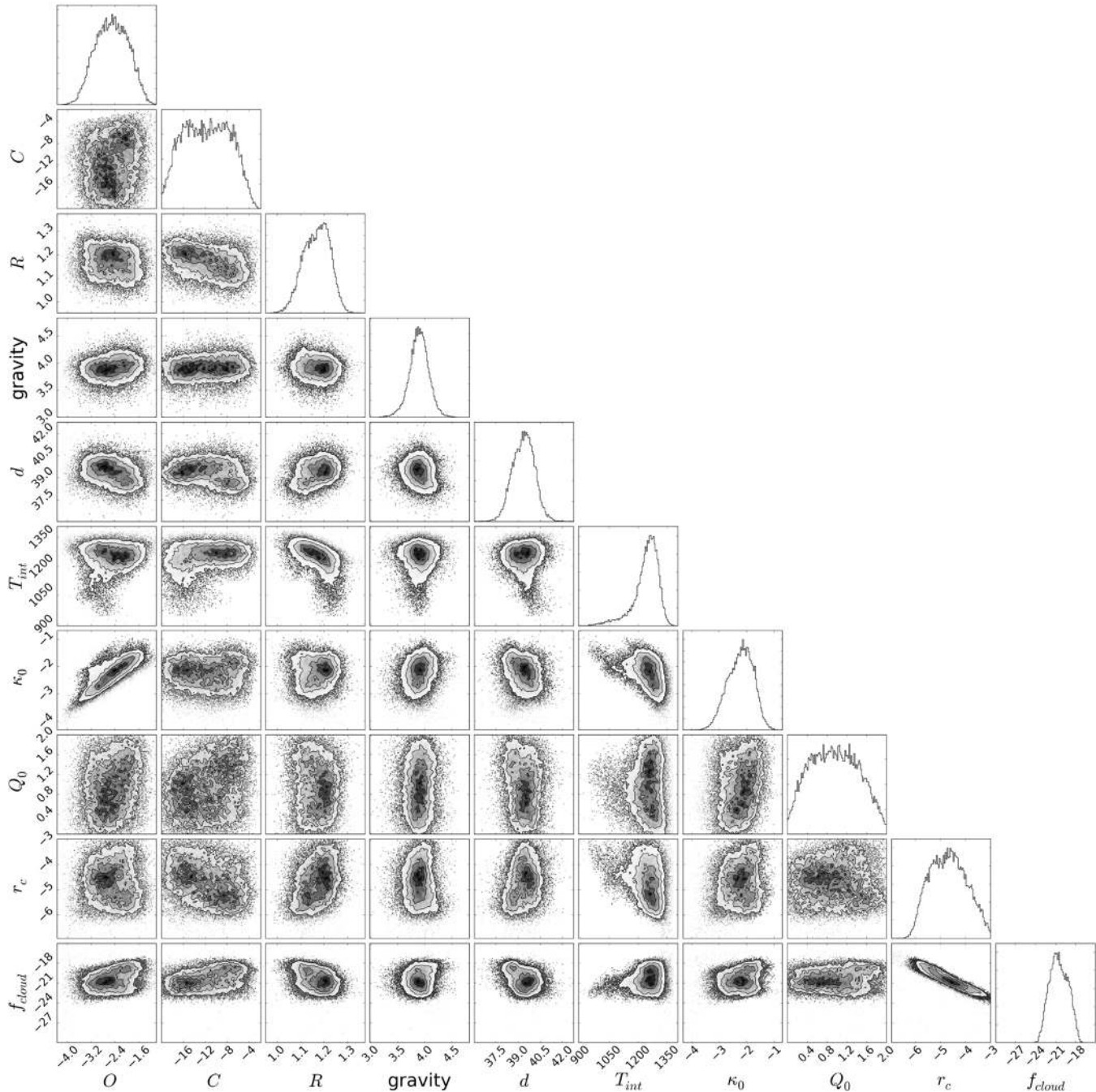
Figure B5. Same as Figure B2, but for HR 8799e.
