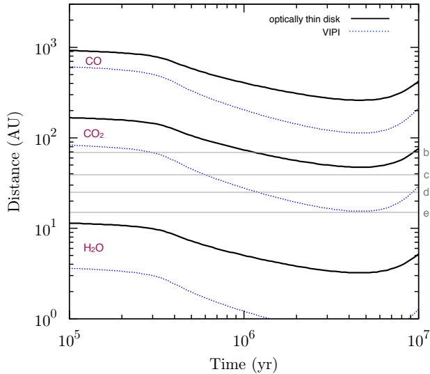
Figure 14. Positions of the CO, CO 2 and H 2 O snowlines or icelines as functions of the stellar age of the HR 8799 system. The solid curves are calculated assuming an optically thin disk. The dotted curves are calculations from a vertically isothermal, passively irradiated (VIPI) disk.
