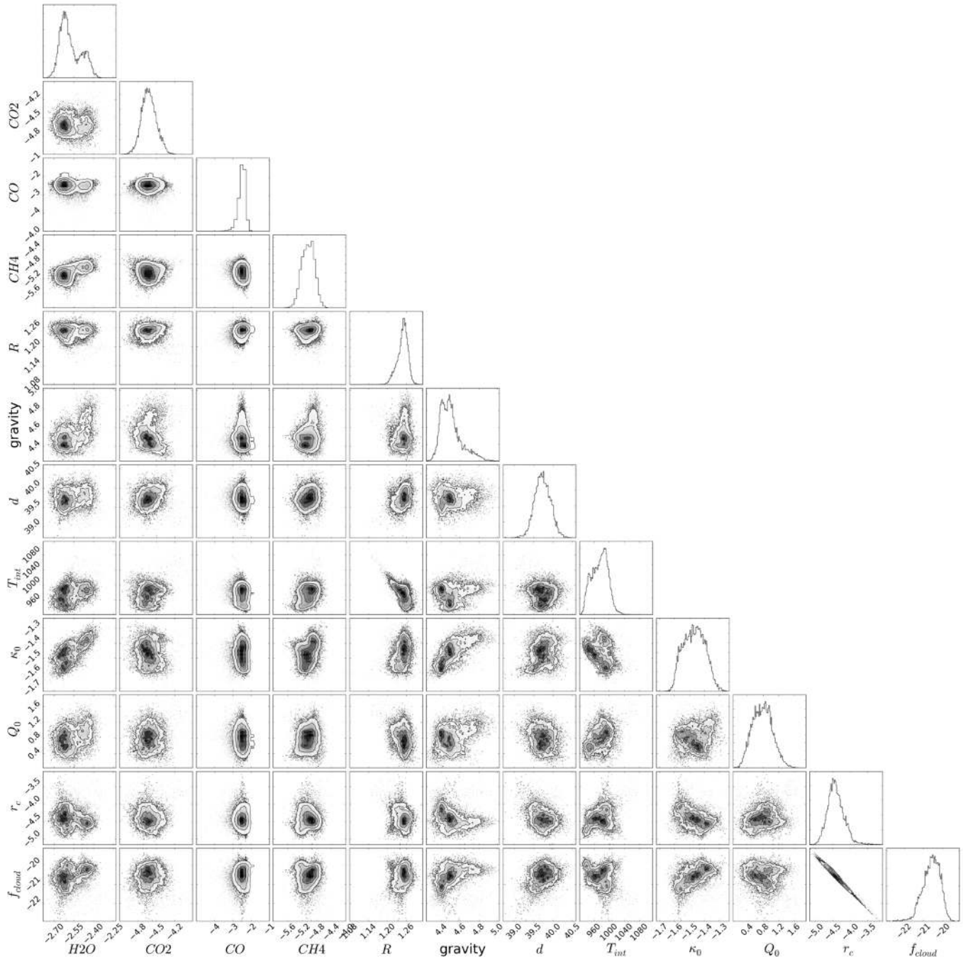
Figure B3. Same as Figure B2, but for HR 8799c.
