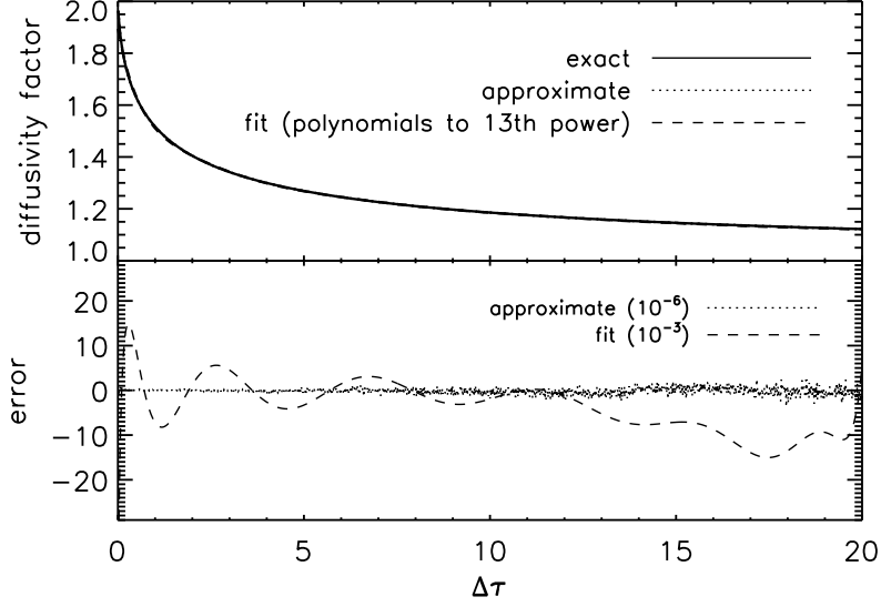
Figure A1. Calculations of the diffusivity factor using a canned routine (“exact”) versus those performed using our fitting formulae for \mathcal{E}_1 in equation (A1) (“approximate”). The calculation labeled “fit” is a 13th order polynomial fit to the exact solution, which performs poorly even at the \sim 10^{-3} level.
