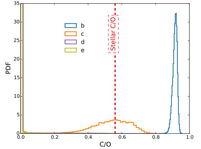
Figure 11. Retrieved C/O values for the HR 8799b, c, d and e directly imaged exoplanets. The stellar C/O value is about 0.56. PDF stands for “probability density function”.
