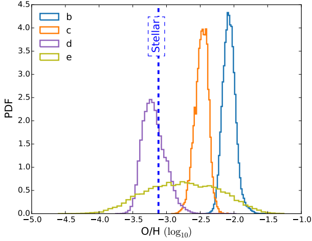
Figure 13. Retrieved O/H values for the HR 8799b, c, d and e directly imaged exoplanets. The stellar O/H value is about 7.6 \times 10^{-4} . PDF stands for “probability density function”.
