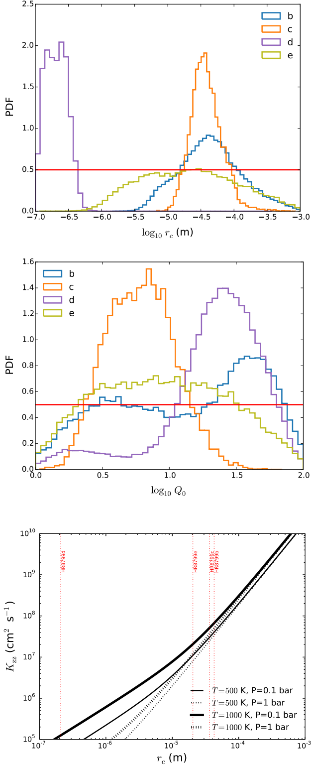
Figure 10. The top and middle panels show the retrieved cloud particle radius and composition parameter for the HR 8799b, c, d and e directly imaged exoplanets, where the flat line is the prior. The bottom panel shows the eddy diffusion coefficient and demonstrates that its inferred value corresponding to the peak value of the posterior distribution for r_c are not unreasonable and broadly consistent with the assumed K_{zz} values in previous studies. PDF stands for “probability density function”.
