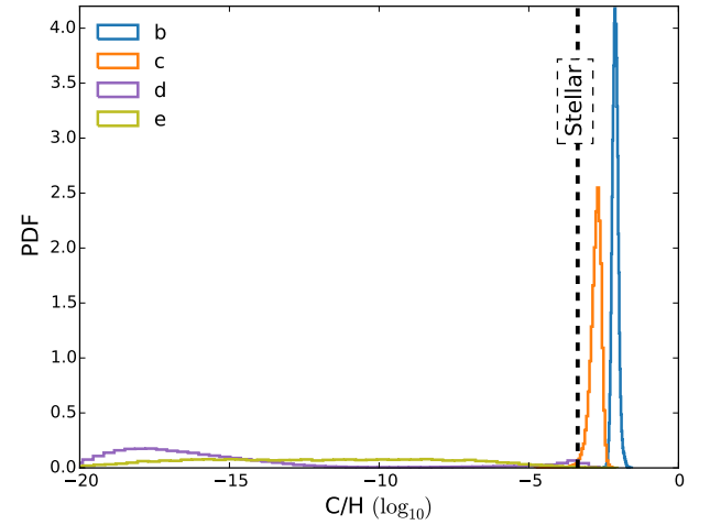
Figure 12. Retrieved C/H values for the HR 8799b, c, d and e directly imaged exoplanets. The stellar C/H value is about 4.3 \times 10^{-4} . PDF stands for “probability density function”.
