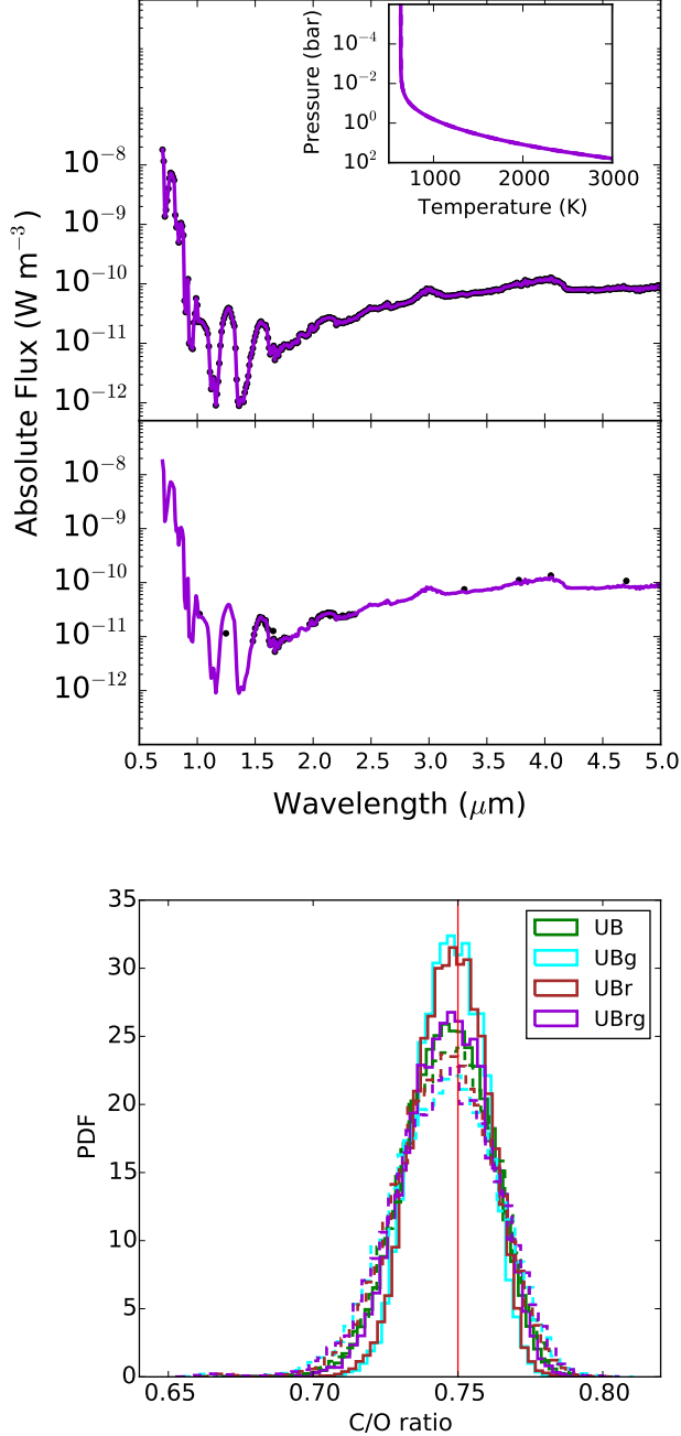
Figure 5. Further results from the retrievals on the mock dataset. The top panel shows the mock dataset at full resolution ( 0.01 \mu\text{m} ), and also with HR 8799b-like data coverage (circles). The mock dataset and best-fit spectrum overlap exactly (to within the resolution of the plot). The insert shows the retrieved temperature-pressure profile. The bottom panel shows the retrieved posterior distributions of C/O assuming different models (see Table 1). The solid and dotted curves are for HR 8799b-like and HR 8799e-like data coverage. The broader posterior distributions of C/O associated with HR 8799e-like data coverage are primarily due to the lack of K band data.
