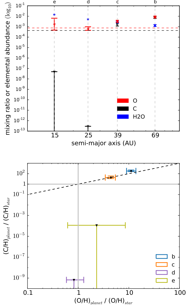
Figure 15. Summary of our main results. The top panel shows the retrieved water mixing ratios and elemental abundances of carbon and oxygen for all four HR 8799 exoplanets. For HR 8799d and e, we show the water abundance in chemical equilibrium at 1 bar (represented by the blue stars). For C/H and O/H, we also show the corresponding values of the HR 8799 star (horizontal dashed lines). The bottom panel shows the exoplanetary elemental abundances normalized to their stellar values with the dashed line denoting parity.
