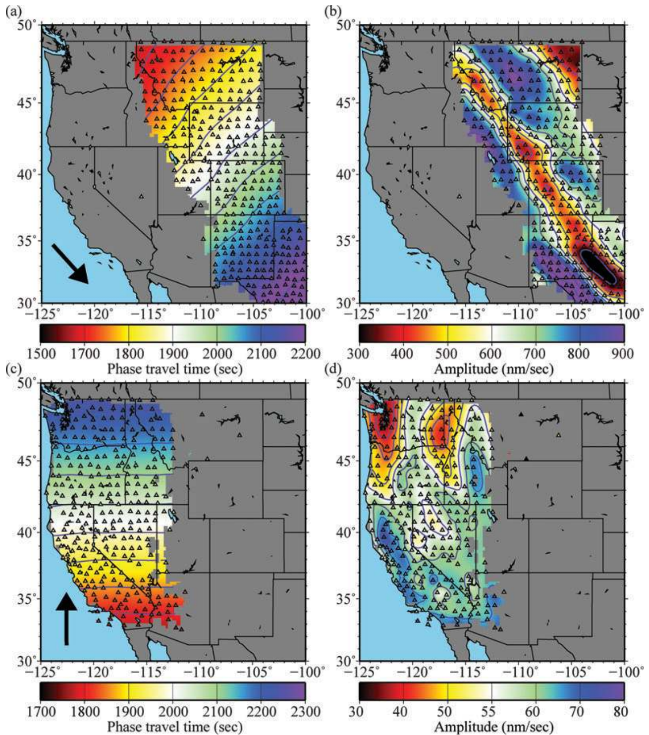
Figure 3. (a)–(b) The 60 s Rayleigh wave observed phase traveltimes and amplitude maps for the 2009 April 7, earthquake near Kuril Islands ( M_s = 6.8 ). The stations with available phase traveltimes and amplitude measurements used to construct the maps are shown as triangles. Contours are separated by intervals of 60 s in (a) and 100 nm s -1 in (b). The arrow in (a) indicates the approximate direction of wave propagation. (c)–(d) Similar to (a)–(b) but for the 2007 February 14, earthquake near Easter Island ( M_s = 5.7 ). Contours in (d) are separated by intervals of 5 nm s -1 .
