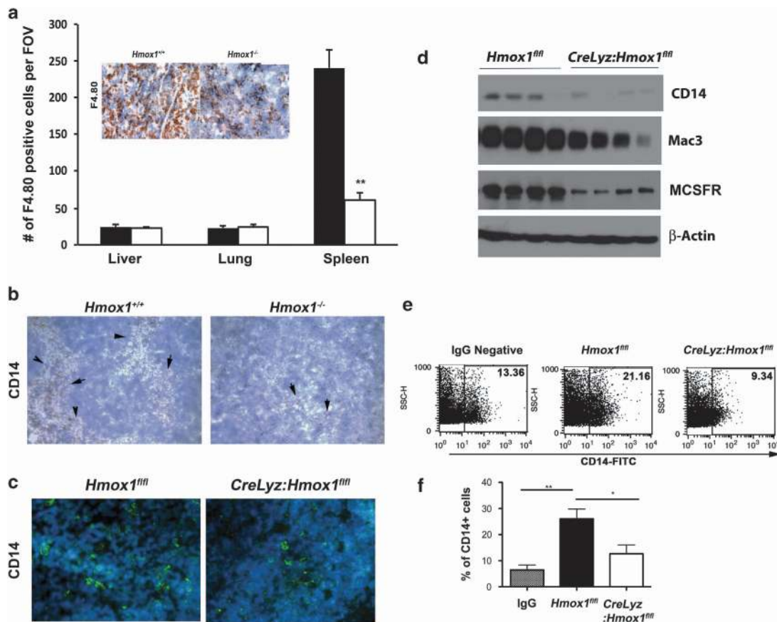
Figure 1 Lack of HO-1 in myeloid cells results in lower number of mature macrophages. (a) Immunohistochemistry with antibody against F4.80 in the spleens, lungs, and livers from Hmxo1 -/- and Hmxo1 +/+ mice. Number of F4.80-positive cells per field of view ( n = 4-6 ) was evaluated. Inset: Representative staining is shown. n = 3 per group. ** P < 0.001 Hmxo1 -/- versus Hmxo1 +/+ . (b) Immunohistochemistry of the spleens from Hmxo1 -/- and Hmxo1 +/+ mice with staining against CD14. Representative sections are shown. (c) Immunostaining with antibodies against CD14 (Alexa-488) was performed on the spleen sections from Hmxo1 fl/fl and CreLyz:Hmxo1 fl/fl mice. n = 3-4 per group. (d) Immunoblotting in the lysates of the spleens from Hmxo1 fl/fl and CreLyz:Hmxo1 fl/fl mice. Antibodies against CD14, Mac3, and MCSFR were applied to test for macrophages maturation. \beta -Actin was used as loading control. n = 4 mice per group. (e, f) Blood cells were isolated by Ficol extraction from Hmxo1 fl/fl and CreLyz:Hmxo1 fl/fl mice ( n = 2-3 per group) and stained against CD14 conjugated with FITC. Appropriate IgG-FITC control antibodies were used. Representative flow cytometry plots are shown in e, and quantitation of fluorescent mean is shown in f. ANOVA, P = 0.0026 ; Tukey's test: ** P < 0.01 Hmxo1 fl/fl versus IgG and * P < 0.05 Hmxo1 fl/fl versus CreLyz:Hmxo1 fl/fl
