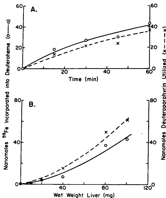
FIGURE 2 Heme synthetase activity in rat liver homogenates. Comparison of ^{59}\text{Fe} incorporation into deuteroheme and deuteroporphyrin disappearance. In A, enzyme activity of homogenates of 50 mg wet wt of liver from a male Wistar rat is shown as a function of time of incubation. In B, incubations were carried out for 45 min, and activity is expressed as a function of the wet wt liver from another male rat. Incubation and assay conditions were as described in Methods.
