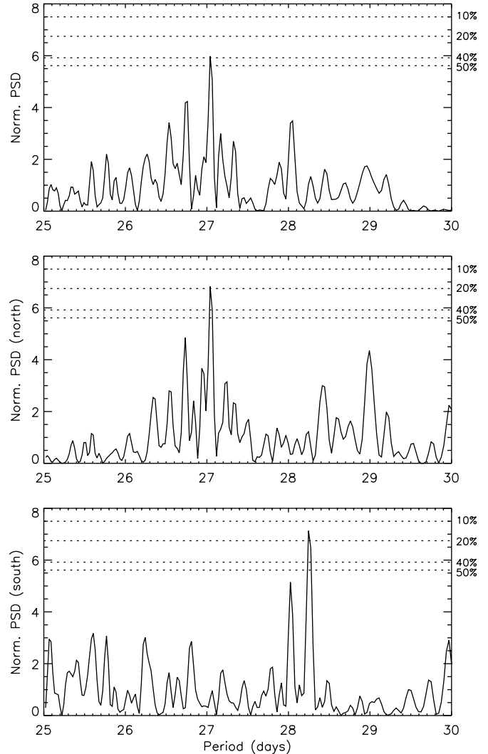
Fig. 7. Periodograms derived from the daily Sunspot Numbers of the total solar disk (top panel), the northern hemisphere (middle panel) and the southern hemisphere (bottom panel), from the time span 1975–2000. The dashed lines indicate various FAP levels.
