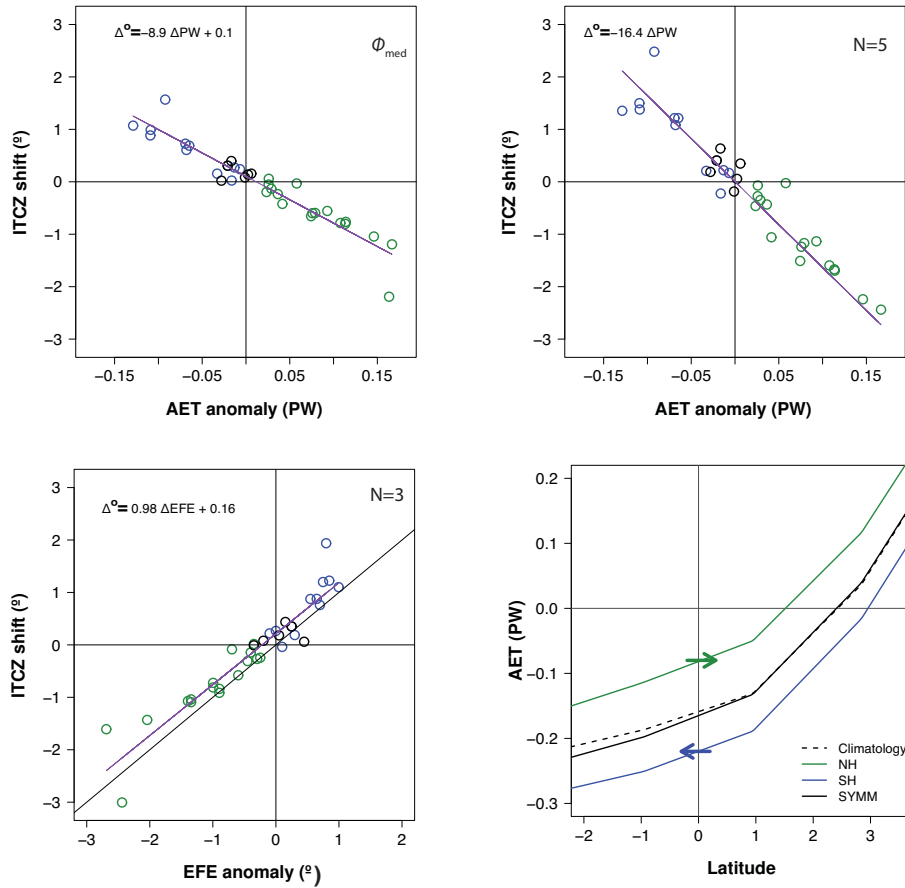
Figure 9. Annual-mean ITCZ shift represented by changes in (top left) \phi_{med} and (top right) \phi_{ITCZ} ( N = 5 ) vs. change in AET_{eq} . Bottom left: changes in \phi_{ITCZ} ( N = 3 ) vs. change in EFE. See text for definitions. Total AET vs. latitude for a small band centered around the equator for all volcanic events in (green) ASYMM_{NH} , (blue) ASYMM_{SH} , and (black) SYMM cases (bottom right). Black dashed line indicates climatological or pre-eruption AET values (different choices are indistinguishable). Colored arrows represent the direction of anomalous AET_{eq} .
