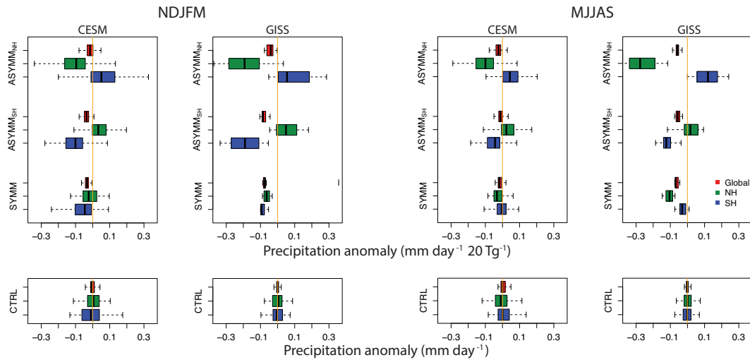
Figure 5. As in Fig. 3, except for precipitation ( \text{mm day}^{-1} , normalized to 20 \text{ Tg} in the forced simulations; \text{mm day}^{-1} in the control). N (not shown) is the same as in Fig. 3.
