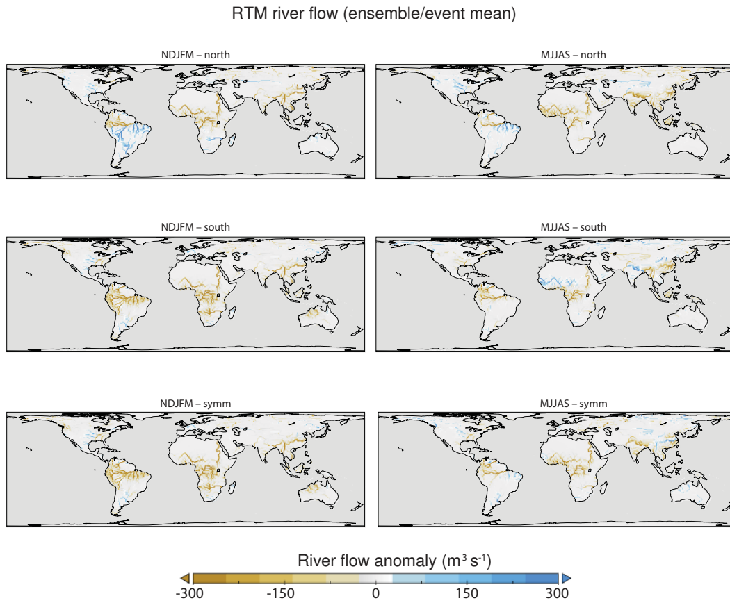
Figure 6. As in Figs. 2 and 4, except for river discharge ( \text{m}^3 \text{s}^{-1} , or 10^{-6} \text{ Sv} ).
