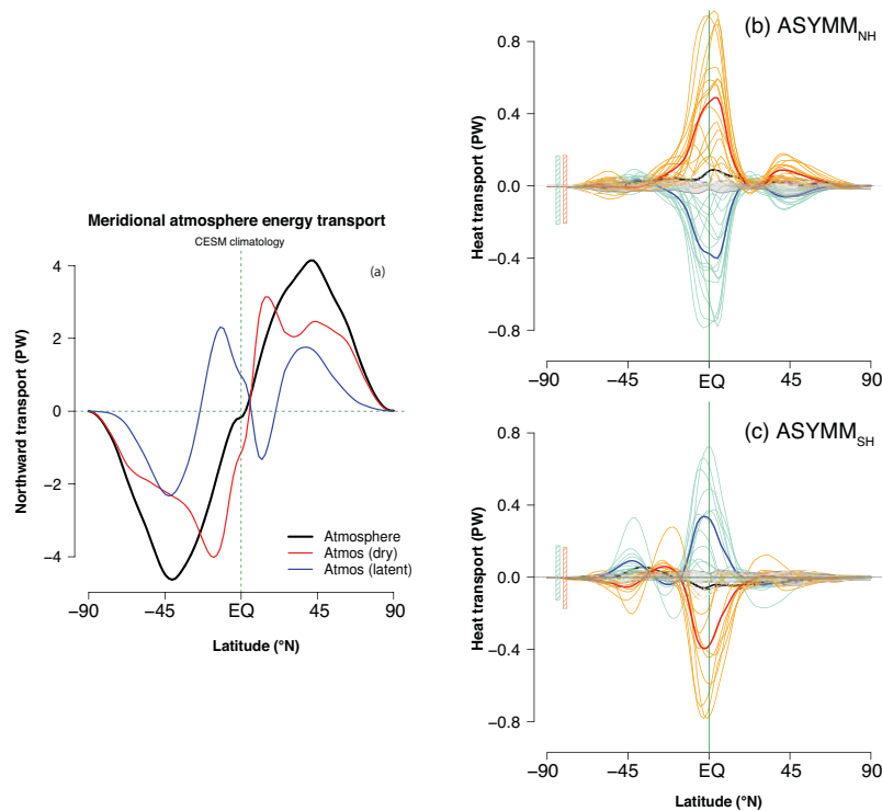
Figure 8. (a) CESM climatology of atmospheric energy transport (PW, black) and dry (red) and latent (dark blue) transports. (b) Composite mean anomaly in atmospheric heat transport for ASYMM NH eruptions in total (black), dry (red), and latent (blue) components. Lighter (orange and aqua) lines represent individual eruptions, each averaged over 17 ensemble members. (c) As in (b), except for ASYMM SH eruptions. Grey envelope corresponds to the total AET anomaly vs. latitude in a control simulation using 50 realizations of a 17-event composite (17 “events” with no external forcing, corresponding to the size of the ensemble). Vertical bars correspond to the range of (aqua) latent and (orange) dry components of cross-equatorial energy transport (AET eq ) in the control composite.
