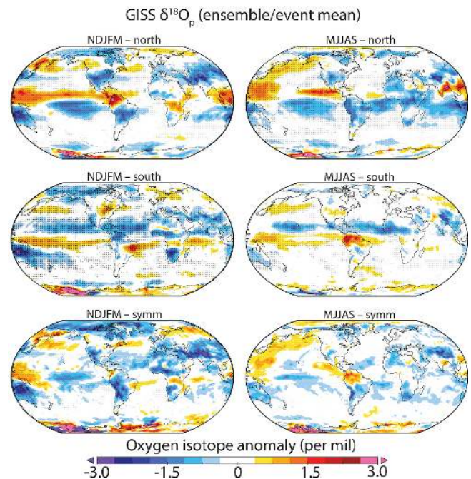
Figure 7. GISS-E2 spatial composite of the oxygen isotope anomaly (‰) in (top row) ASYMM NH , (middle row) ASYMM SH , and (bottom row) SYMM events in (left column) NDJFM and (right column) MJJAS.
