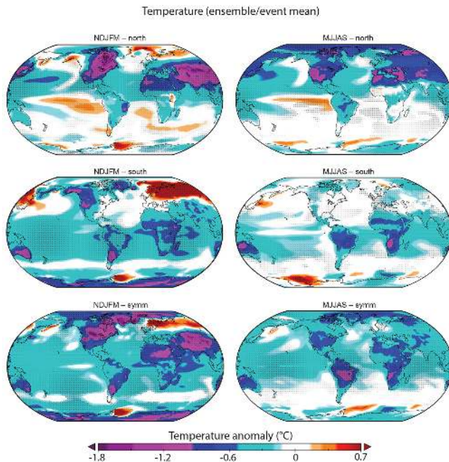
Figure 2. CESM spatial composite of surface temperature anomaly ( ^{\circ}\text{C} ) for (top row) \text{ASYMM}_{\text{NH}} , (middle row) \text{ASYMM}_{\text{SH}} , and (bottom row) SYMM events, each in (left column) NDJFM and (right column) MJJAS. Stippling indicates statistical significance using a two-sided Student's t test ( p < 0.05 ).
