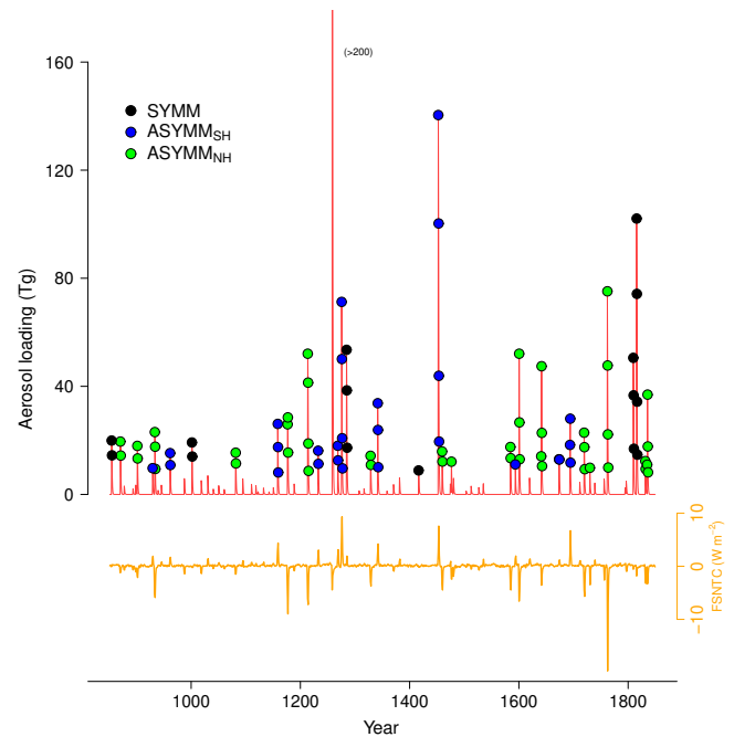
Figure 1. Global aerosol loading (Tg) from Gao et al. (2008) as red line. ASYMM NH (green circles), ASYMM SH (blue circles), and SYMM (black circles) events that are used in composites are shown. Note that Samalás is omitted, as discussed in text. The time series is at seasonal (5-month) resolution, and thus multiple points may be associated with a single eruption. The hemispheric contrast (NH minus SH) clear-sky net solar radiation (FSNTC – in \text{W m}^{-2} ) in CESM LME is shown in orange (offset to have zero mean).
