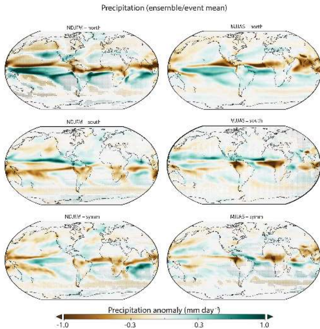
Figure 4. As in Fig. 2, except for precipitation ( \text{mm day}^{-1} ).
