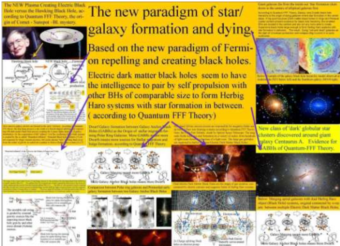
Figure 13, The new paradigm.
