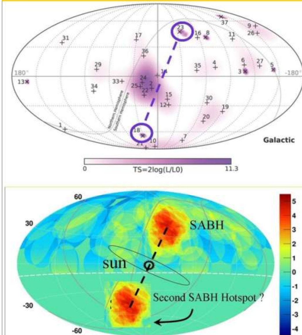
Figure: 11, 9-july 2014. first evidence for the first Solar Anchor Black Hole. (SABH) A hotspot with powerful cosmic rays found under the Big Dipper, by the University of Utah. Now ( 2017) however the southern counterpart ( the second SABH hotspot) is found, See also: http://www.sciencedaily.com/releases/2014/07/140708092910.htm
