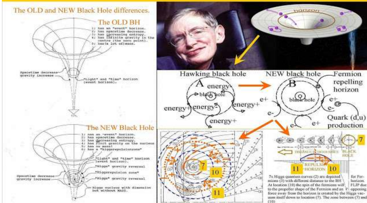
Figure 29, Negative charged Black hole at the outside, positive at the inside originated by the chiral vacuum.
