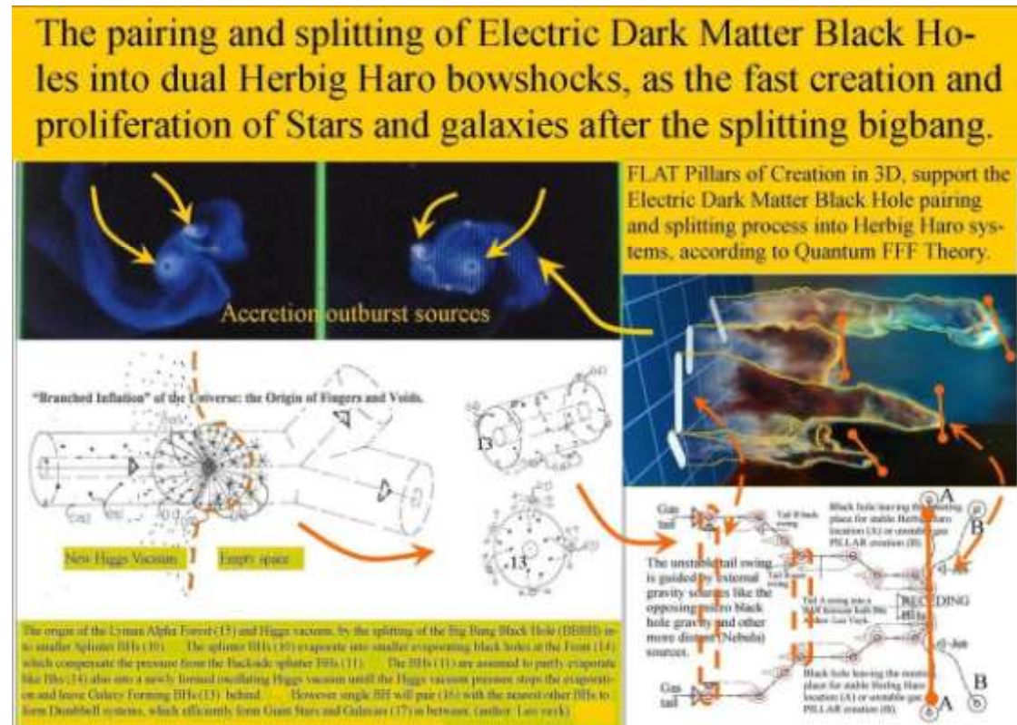
Figure 14, Examples of HH objects and dual DMBH pairing
