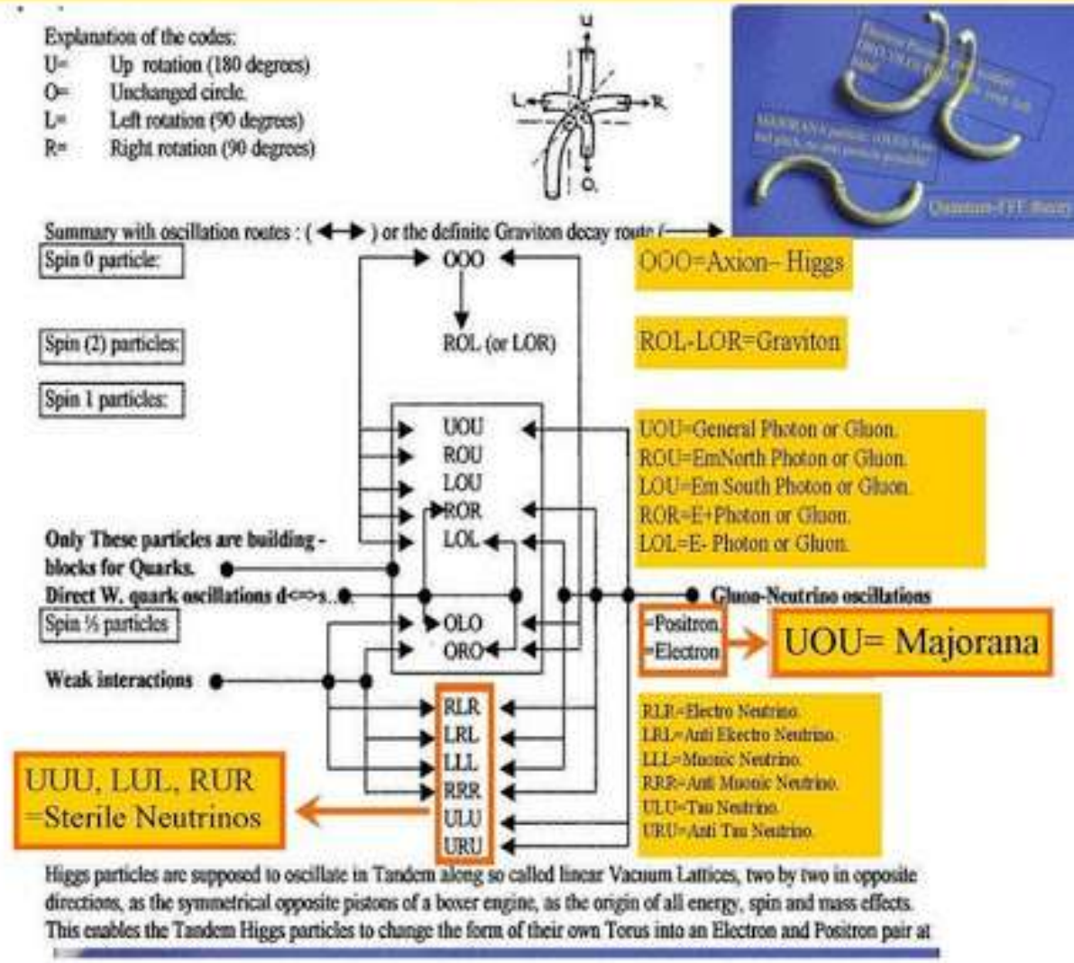
Figure 2, most rigid string particles with much dualities, ( stil undiscovered) described by only three hinges and 4x possible rotations of 90 degrees. (ULRO)
