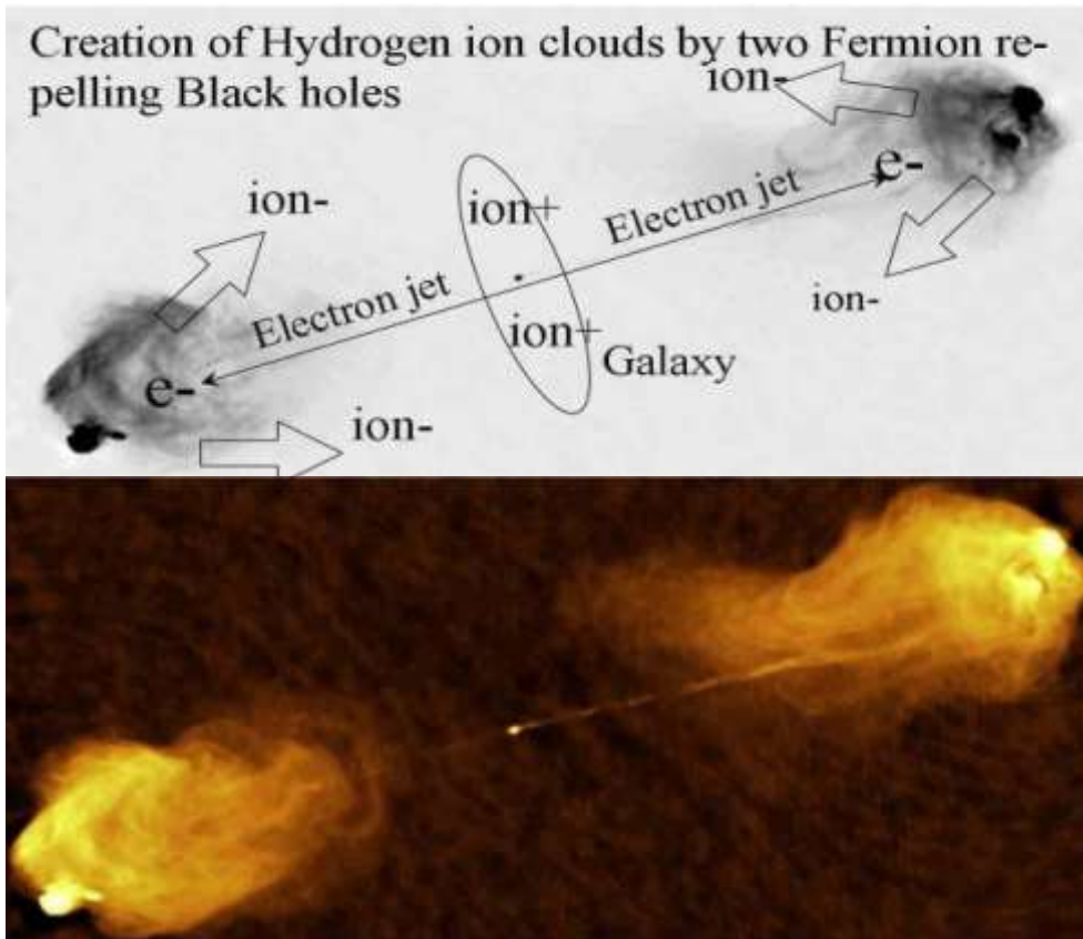
Figure 7, Cygnus A, equipped with Galaxy Anchor Black Holes (GABHs) clear electron jets and Hotspots, showing ionized gas production.
