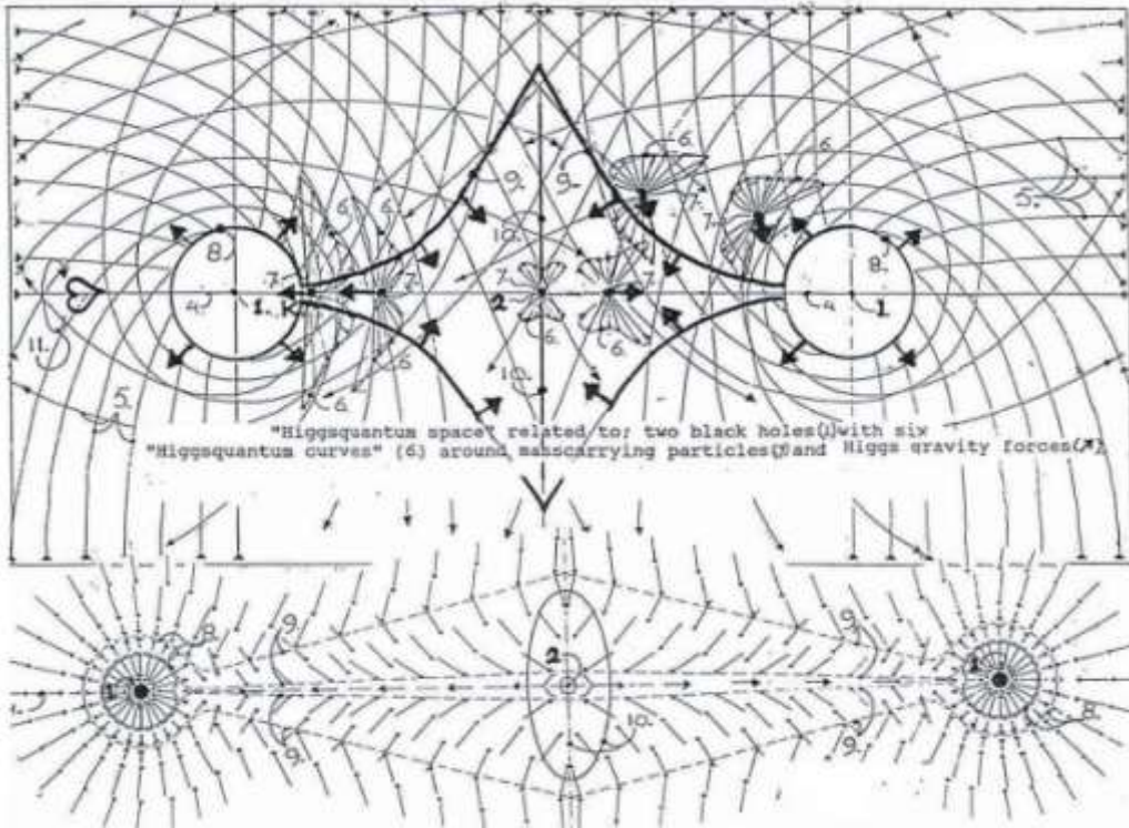
Figure 6, Axion Higgs Vacuum structure around a set of two Black holes, as is found to be present around Planetary nebula and early Galaxies and Herbig Haro objects.
