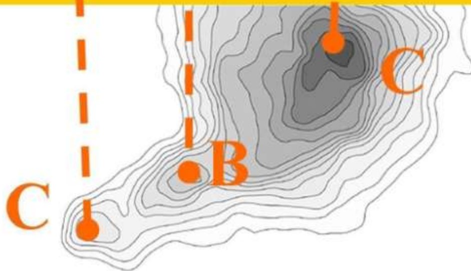
Figure 17, BOK Nebula ESO 9934.
