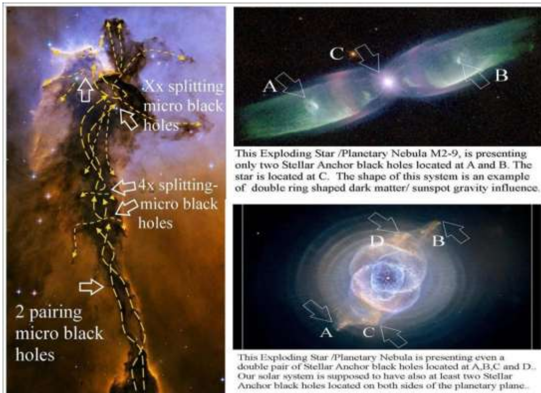
Figure 8, The Spire Eagle nebula, with two Planetary nebula, examples of the importance of black holes in the universe.
