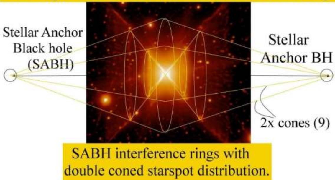
Figure 5, The Red Square Planetary nebula MWC922, equipped with double cone structure of expelled material including trailing starspots (Micro Black Holes). There are FOUR cones of interferences originated by the two Stellar Anchor black holes (SABHs). These four cones seem to interfere with the TWO cones of expelled material of the star, leading to FOUR rings of interference.
