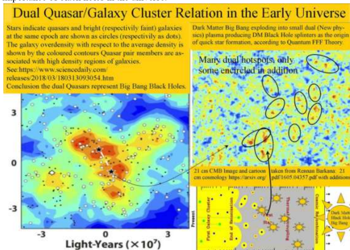
Figure 9, Dual Quasar/ Galaxy and Cluster forming relation in the early universe after Dark Matter Black Hole nuclear Big Bang splitting.
