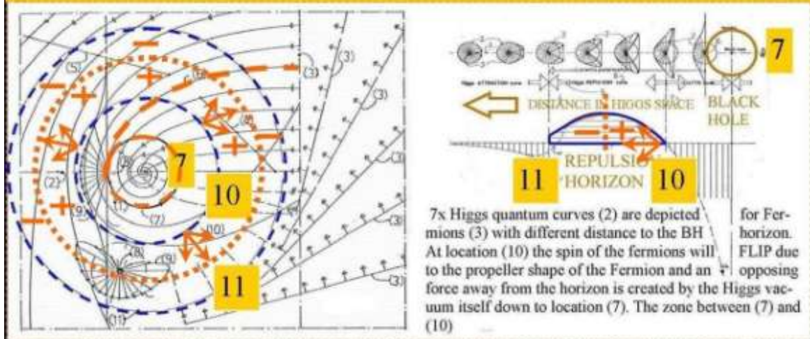
Figure 10, Principle of Fermion repulsion around a black hole according to Quantum FFF theory..
