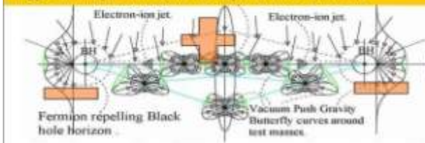
Figure 16, Secondary and Tertiary Dual BH HH systems.
