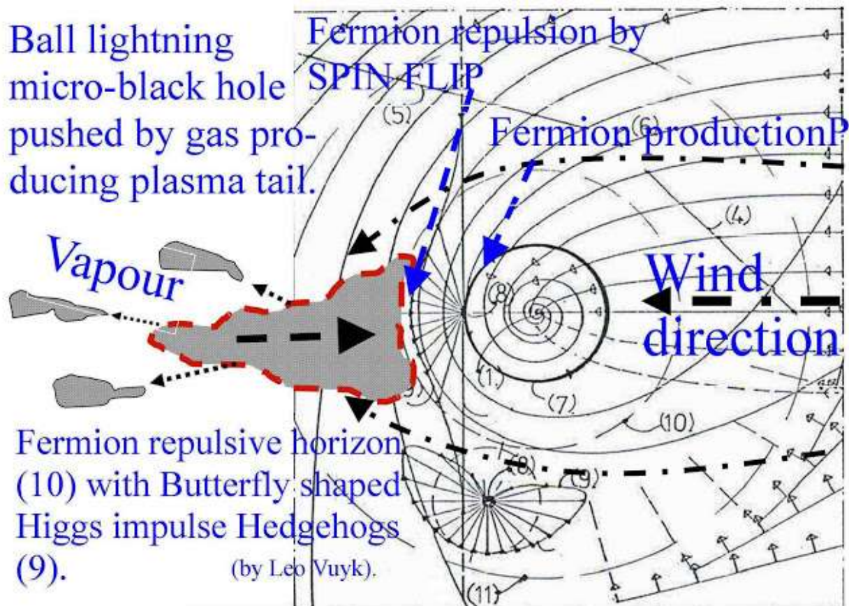
Figure 31, Details of vacuum synchrotron motion around a black hole with plasma creation and tail.
