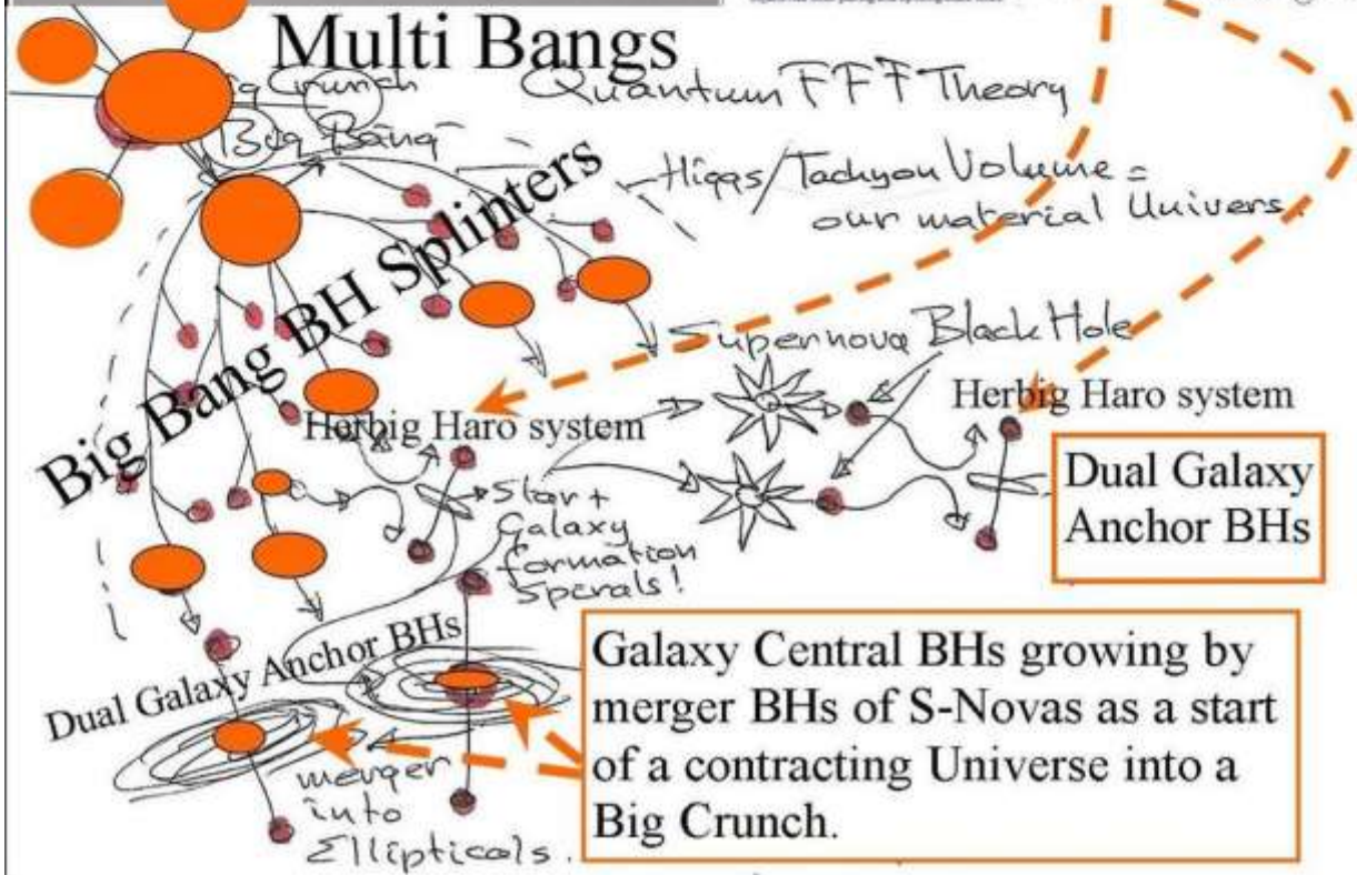
Figure 21, The big Bang splitting of the Dark Matter Black Hole nucleus.
