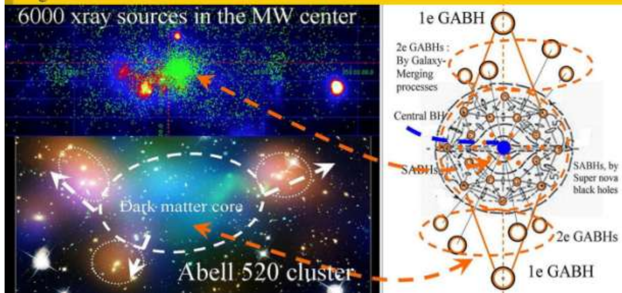
Figure 24, Non inertial Gravitating Dark Matter Black Holes and some specific astrophysical effects.
