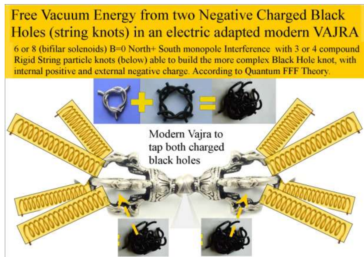
Figure 1, see also: Electric Birkeland Current Production Between Two Herbig Haro Black Holes or even Stable Ball Lightnings on Earth. https://vixra.org/pdf/2002.0094v1.pdf
