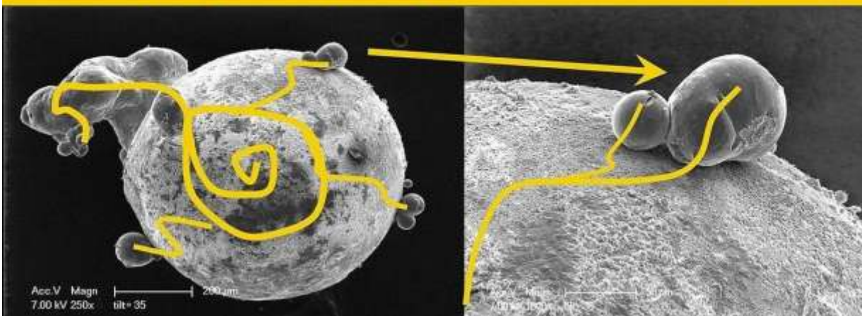
Figure 25. Magnetic Interference microscopic Higgs black holes, ( quantum Knots) with heating effects in silicon and as CERN LHC UFO dust particles.
