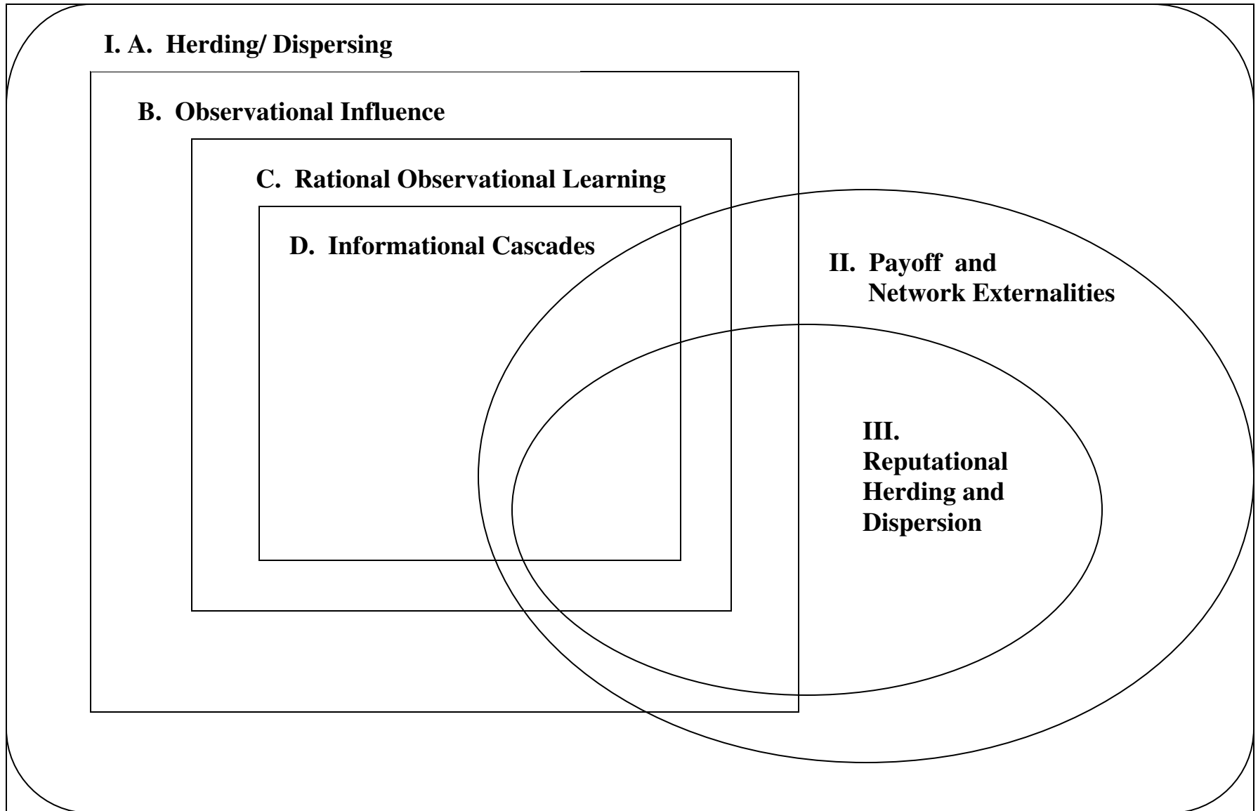
Figure 1: Topic Diagram
