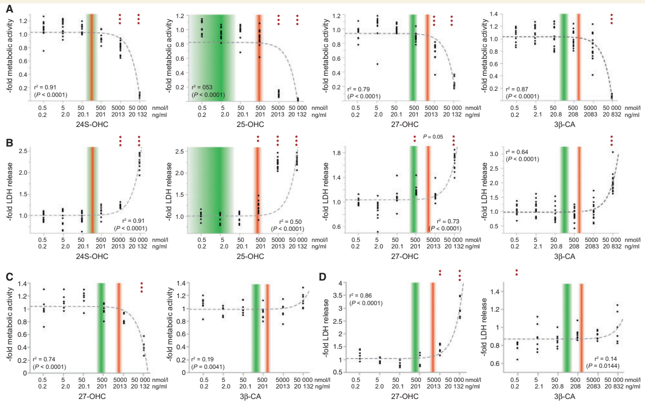
Figure 3 Neurotoxicity of oxysterols. The motor neuron-like cell line NSC-34 ( A and B ) as well as cortical neurons derived from iPSCs ( C and D ) were exposed to increasing concentrations of 24S-OHC, 25-OHC, 27-OHC and 3β-CA. ( A and C ) Metabolic activity was assessed by measuring the cleavage of the tetrazolium salt WST-1 in a colorimetric assay. ( B and D ) LDH-release in the medium was analysed as a measure of cytotoxicity. The range of oxysterol concentration in the serum of healthy controls is indicated by shaded green boxes. Shaded red boxes show the range of values observed in SPG5 patients. Dotted grey lines are fitted following a linear regression model. The horizontal axis is log-scaled.
