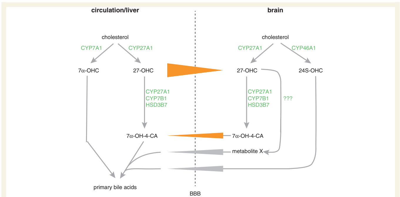
Figure 5 Oxysterol flux across the blood–brain barrier. 27-OHC is produced both in the periphery and the CNS by 27 \alpha -hydroxylation of cholesterol. A net flux of 27-OHC from the circulation to the CNS has been demonstrated (Heverin et al. , 2005), that is most likely driven by the concentration gradient between blood and CSF ( \sim 150 ng/ml 27-OHC in serum versus \sim 0.5 ng/ml 27-OHC in CSF). To eliminate 27-OHC from the CNS, it is metabolized to 7 \alpha -hydroxy-3-oxo-4-cholestenic acid (7 \alpha -OH-4-CA), requiring the action of three key enzymes: sterol 27-hydroxylase (CYP27A1), oxysterol 7 \alpha -hydroxylase (CYP7B1), and 3 \beta -hydroxy-C27-steroid dehydrogenase/isomerase (HSD3B7). 7 \alpha -OH-4-CA is transferred efficiently across the blood–brain barrier (Meaney et al. , 2007). However, the flux of 7 \alpha -OH-4-CA from the brain is too low as to fully explain the elimination of 27-OHC from the CNS (Meaney et al. , 2007). Further routes to metabolize and excrete 27-OHC to the circulation therefore have to be assumed (see ‘metabolite X’ in the figure). BBB = blood–brain barrier.
