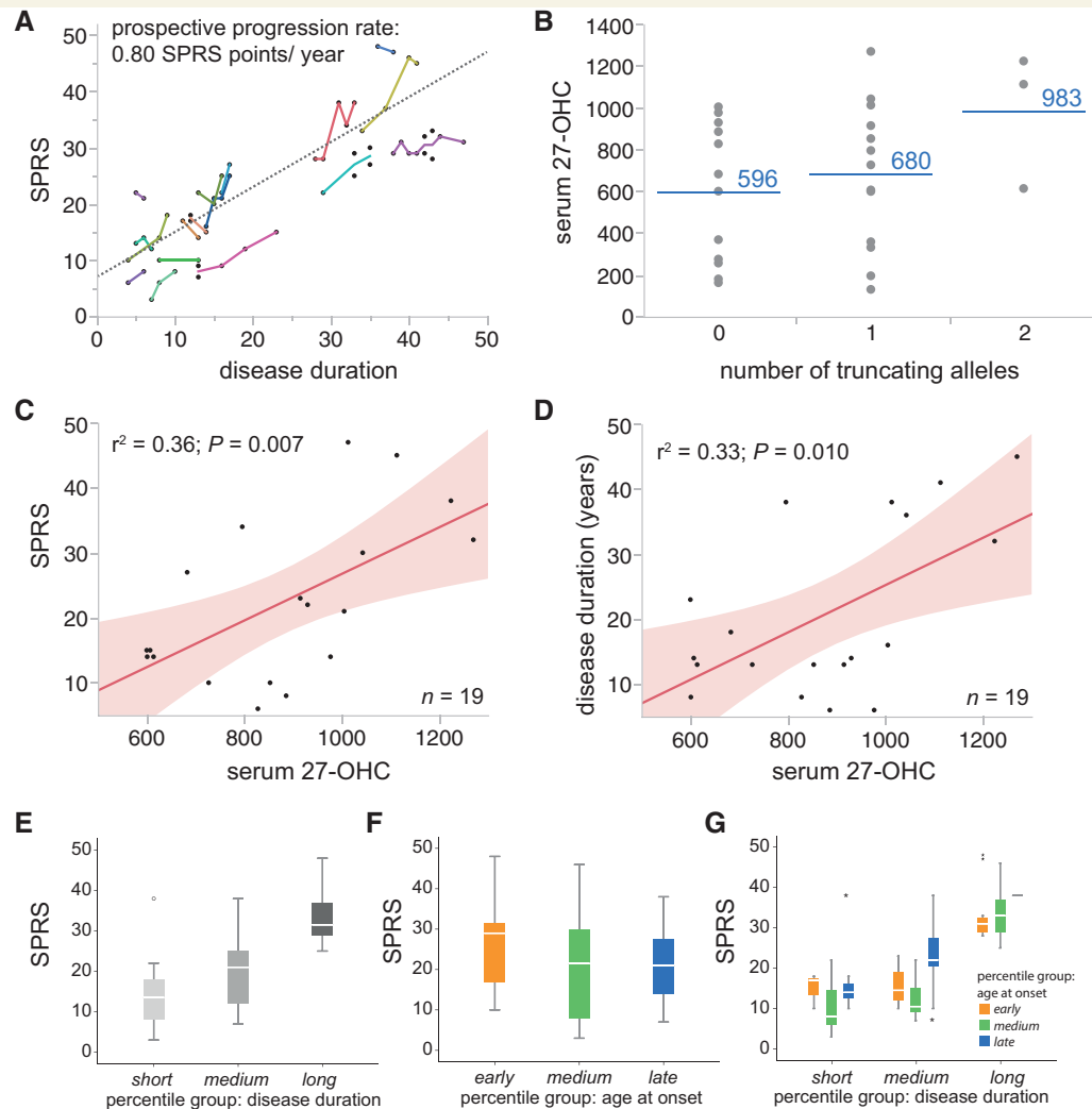
Figure 2 Longitudinal disease progression rate, factors influencing disease severity and oxysterol association with clinical parameters. (A) Longitudinal follow-up examinations in 21 SPG5 patients over a median follow-up interval of 12.4 months. The superimposed dotted grey line indicates the prospective progression rate of 0.80 SPRS points per year; derived from a linear mixed model with SPRS score as dependent variable and disease duration at examination as fixed effect. (B) Levels of 27-OHC (in serum) in dependence on the mutation type. Patients that carry missense mutations on both alleles have lower levels of 27-OHC in serum than cases with mono- or bi-allelic truncating mutations. Blue lines indicate median 27-OHC levels in serum. (C and D) Higher levels of 27-OHC in serum are associated with more severe disease and explain 36% of the variability of the SPRS score ( P = 0.007 ). In cross-sectional data obtained from 19 SPG5 patients serum 27-OHC levels are furthermore higher at later disease stages ( r^2 = 0.33 ; P = 0.010 ). (E) Disease severity increases with longer disease durations. Groups 'short', 'medium' and 'long' correspond to subgroups of the total cohort classified into tertiles ( n = 19 ). (F) No differences of disease severity are observed depending on age of onset tertiles when considering the total cohort ( n = 19 ). (G) In the subgroups with medium and long disease duration, later onset is associated with more severe disease ( n = 19 ).
