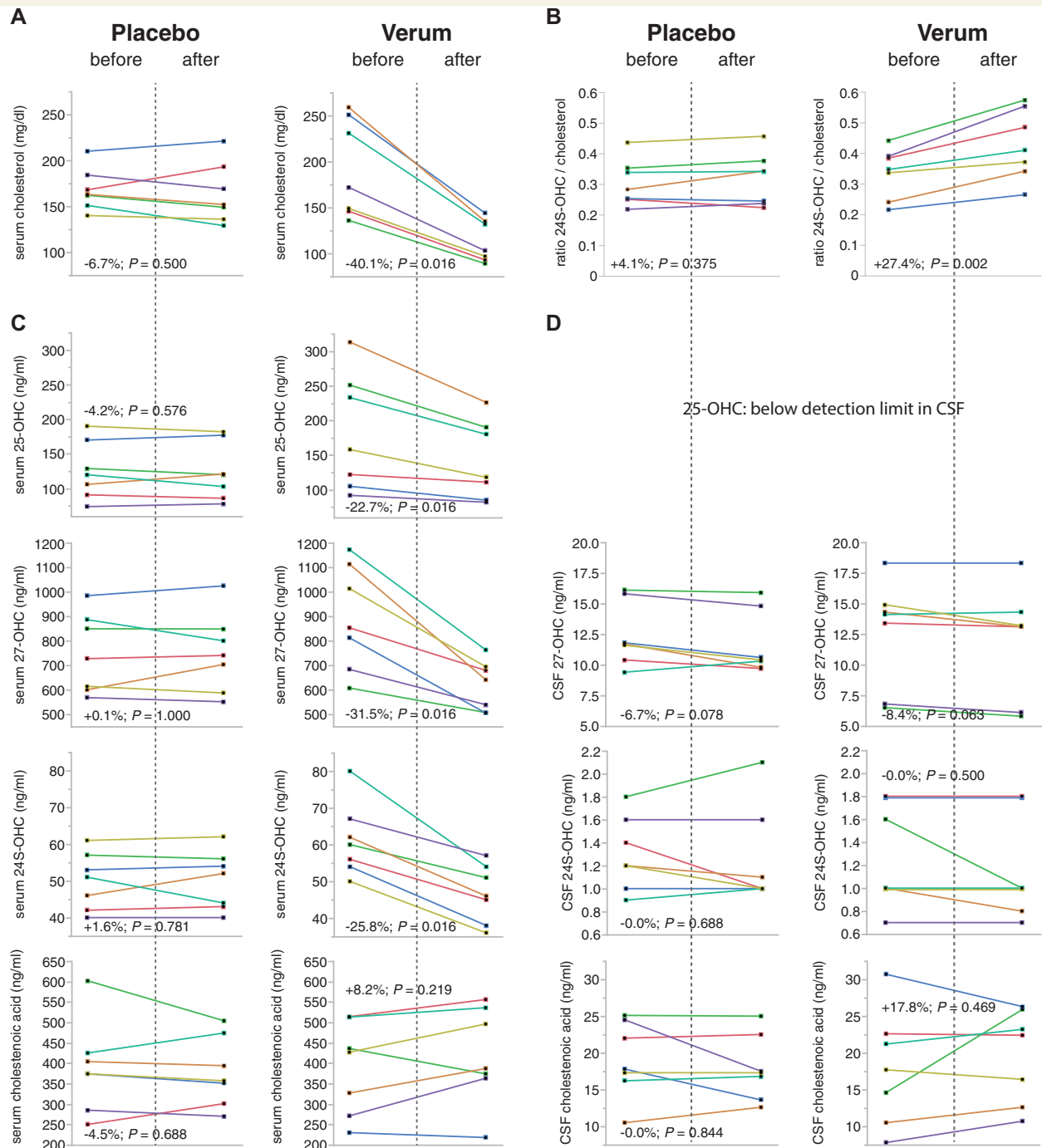
Figure 4 Individual treatment responses. Individual levels of cholesterol and oxysterols before and after treatment with placebo (left column) or atorvastatin (right column). Data from serum analyses are given in (A and C) and for CSF in D. The mean change of values across the group and the P -value for a sign rank test is given for each analyte. The ratio between brain-derived 24S-OHC and cholesterol (B) can be used as an indirect indicator of station effects on brain cholesterol metabolism (Thelen et al. , 2006).
