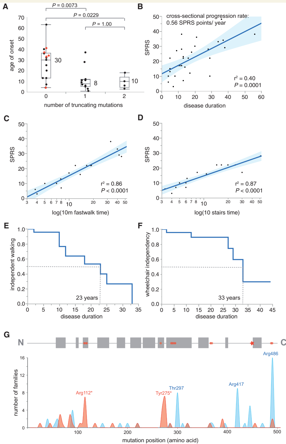
Figure 1 Cross-sectional and time-to-event analyses of disease severity and progression. (A) Age of onset distribution: patients with bi-allelic missense mutations had a later age of onset [median 30 years (IQR 13–37)] than those with either one [median 8 years (IQR 5–12)] or two [median 10 years (IQR 5–14)] truncating mutations (Mann-Whitney U-test, two-sided). The median age of onset in the total cohort was 13 years (IQR 6–32). Patients carrying the Arg486Cys mutation on both alleles are marked by red dots. With the exception of one case (Patient F10.1), all carriers of the homozygous Arg486Cys mutation manifested beyond the age of 30 years. Notably, all carriers of an Arg486Cys allele, which has a minor allele frequency of 0.1% in the European population while it is absent in the Latino population, were of European descent. (B) SPRS score by disease duration: disease severity as measured by the SPRS strongly correlated with disease duration in this cross-sectional cohort of SPG5 cases ( n = 31 ). The fitted cross-sectional progression rate (SPRS points per year with the disease) is 0.56 points/year. The 95% confidence interval of the modelled fit is shaded in blue. (C) Fast walk (10 m) by SPRS: the time needed to cover a 10 m distance on a flat surface including one turn (item 3 of the SPRS) strongly correlated with the SPRS ( n = 19 ). The best fit was reached after logarithmic transformation of
