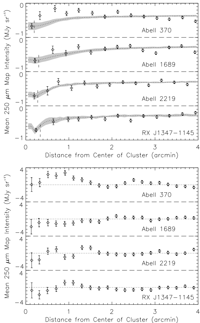
Figure 2. Intensity profiles toward four clusters, illustrating gravitational lensing of the CIB. The left-hand plots show the mean flux density in 0'.25-wide annular bins for each cluster after all detected sources have been removed. The central data point is constructed from averaging map pixels within the effective radius characteristic of the clusters' critical lines (marked by the vertical dashed lines). At larger radii, the data points represent uncertainty-weighted averages starting at the characteristic critical line radius. The mean level of each simulated map is constructed to be zero before source subtraction and is reduced by \sim 0.3 MJy \text{sr}^{-1} after a large fraction of the CIB has been detected as sources and removed; the offset varies between targets depending on the details of the catalog. The uncertainties on the data points reflect the photometric accuracy of the measurements rather than the precision with which the mean should differ from the model. The dotted lines and grey contours show the mean and standard deviation of our sky model, calculated from simulations of the CIB lensed by each cluster and passed through our data analysis pipeline. The right-hand plots show the annular averages of the raw cluster images with no source extraction, which highlight the structure of the surface brightness which is subtracted by removing detected sources.
