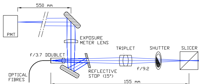
Fig. 3. Optical fibres entering the spectrograph, focal-ratio-adaptation optics, exposure metre and slicer.
