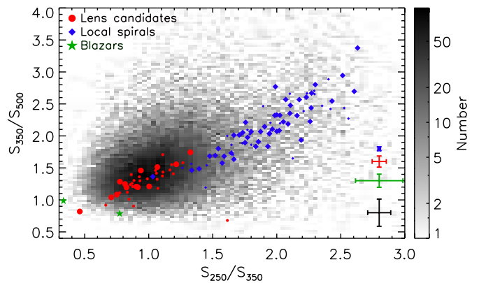
Figure 2. SPIRE color-color diagram for sources detected in HerMES blank fields. Candidate lensed galaxies, blazars, and bright local spirals are highlighted; large and small symbols signify sources with S_{500} > 100 mJy and S_{500} = 80\text{--}100 mJy, corresponding to the principal and supplementary samples, respectively. The gray-scale data show the density of all HerMES sources in these fields. The lensing candidates have submillimeter colors that are consistent with the rest of the SPIRE population. Median error bars for each population are shown at the bottom right.
