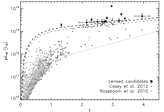
Figure 4. Apparent rest-frame 8–1000 \mu\text{m} infrared luminosity as a function of redshift for HerMES sources, assuming no lensing magnification . Large and small symbols represent our principal and supplementary candidates, respectively. Due to the selection of the brightest 500 \mu\text{m} sources, the candidate gravitationally lensed galaxies appear significantly more luminous than a comparison sample of “normal” (assumed not to be lensed) HerMES sources (Roseboom et al. 2010; Casey et al. 2012). The curved lines represent the approximate selection limits for the samples; the two upper lines (dashed) represent the candidate lensed SMG selection and are the luminosities of an optically thin, T_{\text{D}} = 35 K modified blackbody with observed 500 \mu\text{m} flux densities of 100 and 80 mJy (thick and thin, respectively, corresponding to the principal and supplementary candidates, respectively). The lower line (dotted) represents the selection of sources in the two comparison samples, as described in the text. Error bars are omitted from the supplementary candidates and the comparison samples for clarity.
