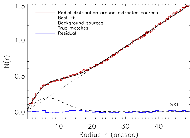
Figure 3. The radial distribution of positional offsets between extracted sources and input sources per extracted source (red line), the best-fitting model prediction (black solid line) and the difference between the two (blue line). The radial distribution of background input sources uncorrelated with the extracted source grows linearly with r . The radial distribution of true matches between the input and output follows a Rayleigh distribution. Note that in this plot we use the SXT 350 \mu\text{m} catalogue extracted from the unclustered simulation of the COSMOS field.
