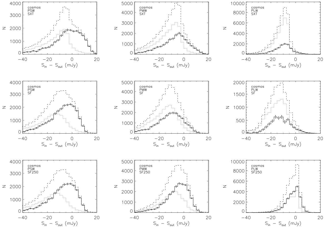
Figure 4. The flux difference distribution of all matches between the input and output (dashed histogram) in the simulated unclustered COSMOS field, between the input and randomized output (dotted histogram), and the difference between the two (solid histogram) for SXT (top panels), SF (middle panels) and SF250 (bottom panels) catalogues. Each column corresponds to a different band (left: 250 \mu\text{m} , PSW; middle: 350 \mu\text{m} , PSW; right: 500 \mu\text{m} , PLW).
