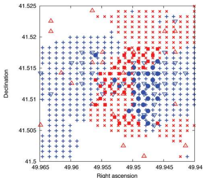
Figure 6. The kinematics of the three phases, optical, FIR and millimetre, represented by H\alpha , [C\ II] and CO(2-1) line emissions, respectively. Shown are the redshifted (red symbols) and blueshifted (blue symbols) velocities for the three phases. The [C\ II] velocities are shown as plus (blueshifted) and cross (redshifted) symbols, the H\alpha velocities are shown as filled circles (blueshifted) and squares (redshifted) and CO(2-1) velocities are shown as open down-triangles (blueshifted) and up-triangles (redshifted).
