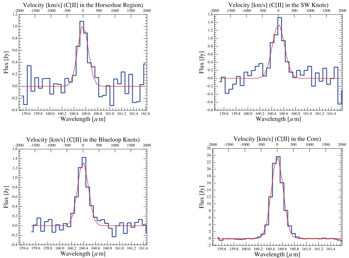
Figure 4. The [C\ II] emission from the Horseshoe knot in the NW (upper-left panel), the SW1/SW2 knots in the SW (upper-right panel) and the Blue Loop knots in the SE (lower-left panel). These apertures are marked in Fig. 3. We also show the [C\ II] spectrum for the core region (lower-right panel), marked in the upper-left panel of Fig. 5.
