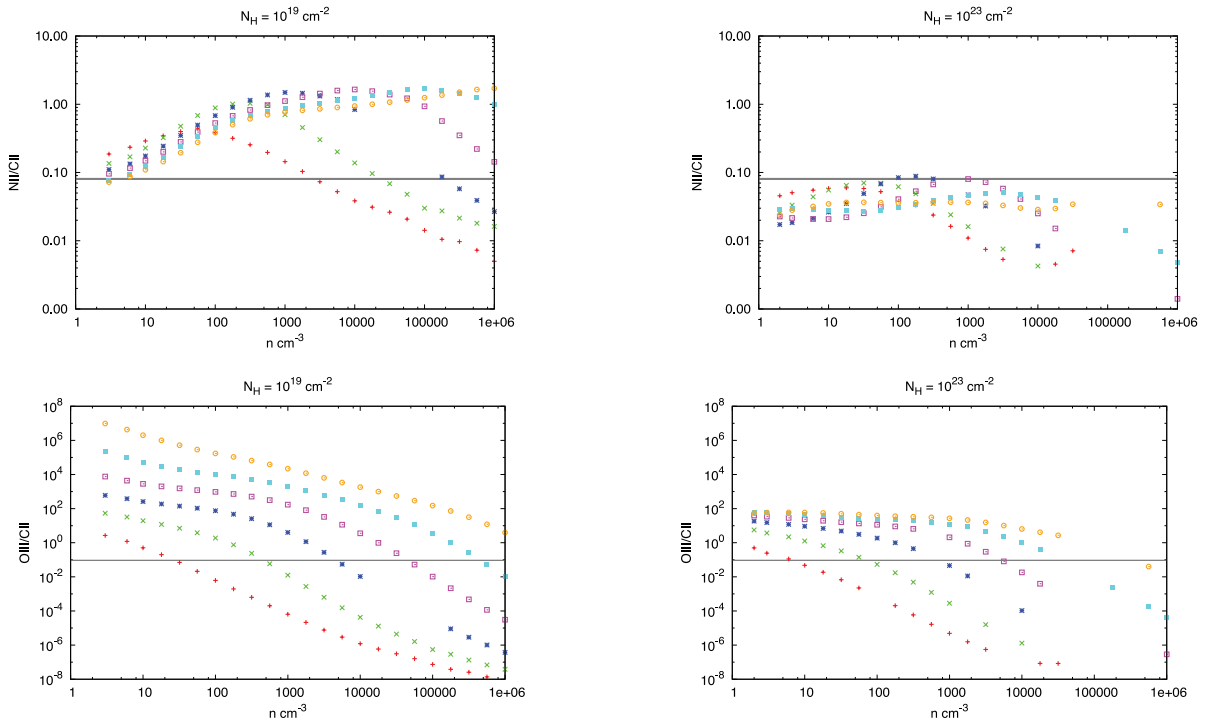
Figure 13. [N II]/[C II] (upper row) and [O III]/[C II] (lower row) versus density, n . Shown are the ratios for two different column densities, N_{\text{H}} = 10^{19} (left) and 10^{23} \text{cm}^{-2} (right). [N II] and [O III] are produced in abundance at the surface of the cloud facing the ionization source and deplete with the depth of the cloud and, hence, sensitive probes of N_{\text{H}} . The different points have the same meaning as in Fig. 12. The horizontal lines represent the observed ratios in the inner 4 kpc region.
