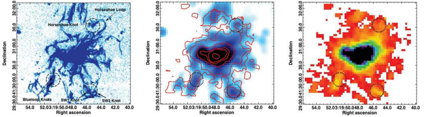
Figure 3. Left: the continuum-subtracted WIYN H\alpha line emission with a spatial resolution of 0.6 to 0.8 arcsec (Conselice et al. 2001). Middle: the H\alpha image smoothed to the resolution of [C\ II] , with the [C\ II] line contours overlaid in red. Right: the Herschel [C\ II] line emission with a spatial resolution of 11 arcsec (this work). The optical H\alpha emission and IR [C\ II] emission show a remarkably similar distribution. Marked are the Horseshoe knot in the NW 20 kpc from the BCG, the SW1/SW2 knots in the SW 21 kpc from the BCG and the Blue Loop knots in the SE 16 kpc from the BCG.
