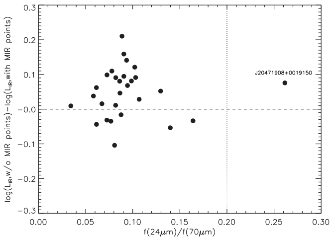
Figure 4. Differences between L_{\text{IR}} using the DL07SED fitting without and with MIR fluxes vs. MIR-to-FIR color: f(24\ \mu\text{m})/f(70\ \mu\text{m}) , for H-KPAIR spiral galaxies with Spitzer observations by Xu et al. (2010).
