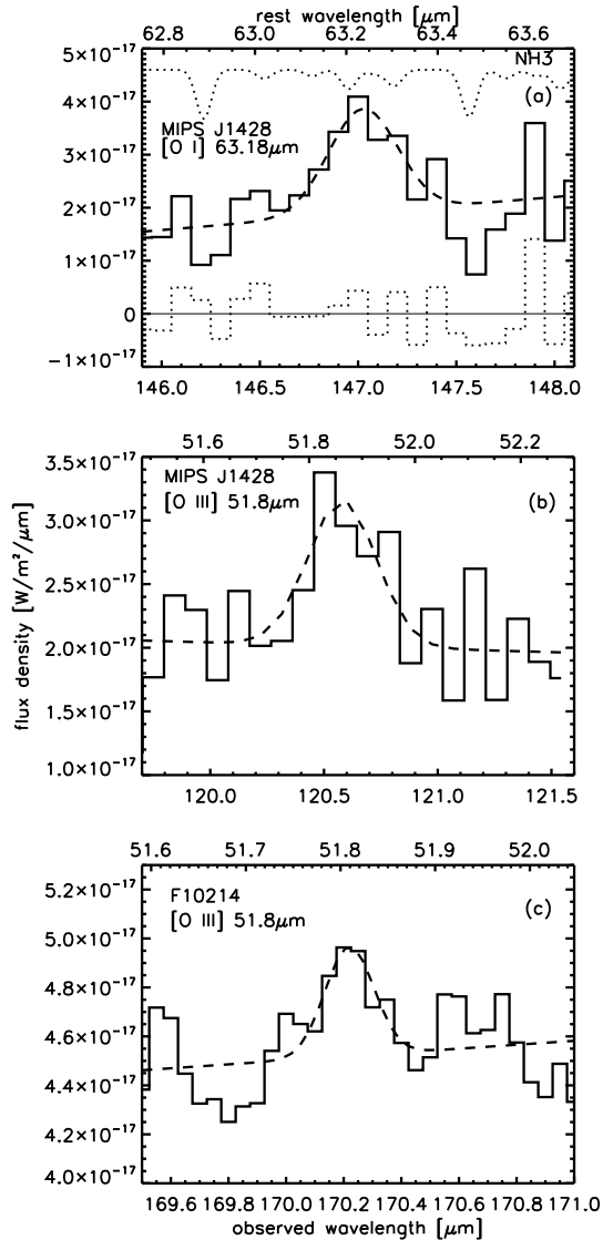
Fig. 1. Observed PACS spectra. Top: [O I]63.2 \mu\text{m} in MIPS J1428. Overplotted is a Gaussian profile on top of a linear continuum fit. Also shown (upper dotted line) is a \text{NH}_3 model (arbitrarily scaled), and the residual (lower dotted line) after subtracting the line+continuum+ \text{NH}_3 fit from the data. Middle: [O III]51.8 \mu\text{m} in MIPS J1428. Overplotted is a gauss profile on top of a linear continuum fit. Bottom: [O III]51.8 \mu\text{m} in F10214. Overplotted is a gauss+linear continuum fit.
