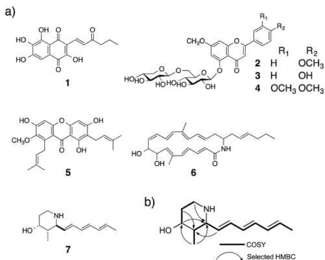
Fig. 3 (a) Structures of isolated natural products 1–7. (b) Key 1 H– 1 H-COSY and HMBC data for 7.
