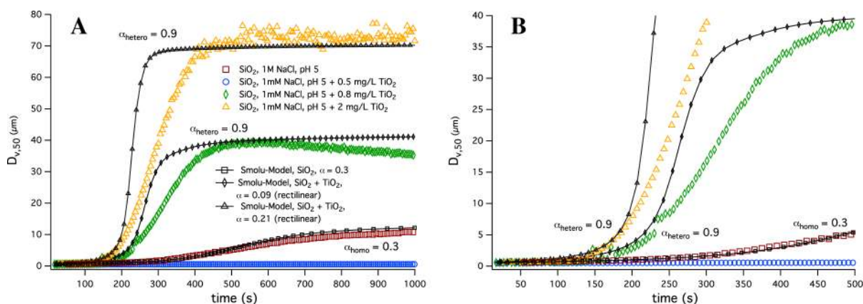
Figure 2. (A) Example of analysis of aggregation data with the Smolu-Model for homoaggregation of 100 mg/L \text{SiO}_2 and heteroaggregation of 100 mg/L \text{SiO}_2 and \text{TiO}_2 at pH 5. (B) Zoom into the initial aggregation stages.
