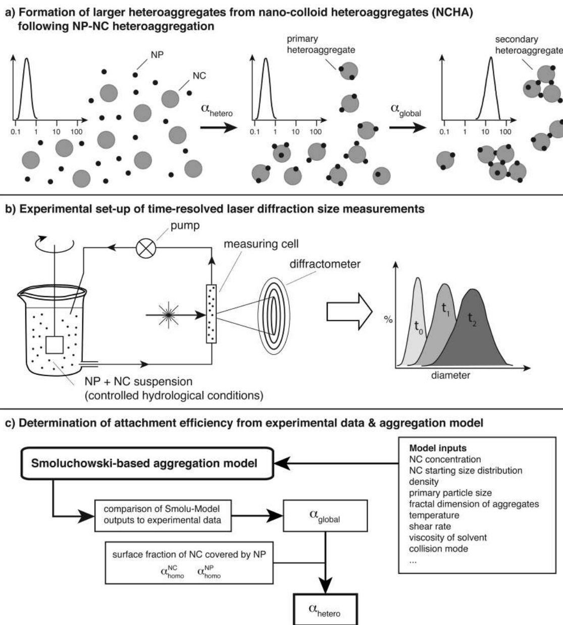
Figure 1. Overview of the general concept developed in this study to determine attachment efficiencies for heteroaggregation, \alpha_{\text{hetero}} . (a) The aggregation of small NPs with larger NCs, first forming NP-NC primary heteroaggregates which then further aggregate with each other to form larger secondary heteroaggregates. (b) Experimental setup. (c) The data interpretation with an aggregation model and calculation of \alpha_{\text{hetero}} is visualized.
