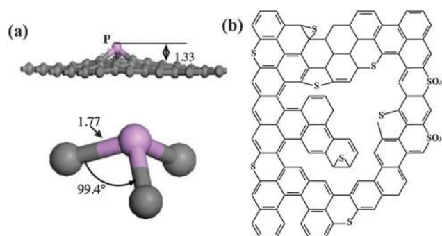
Fig. 12 (a) Optimized geometrical structure of P-doped graphene. The gray and pink balls represent the carbon and phosphorus atoms, respectively. The bond distances are in angstroms. Adapted with permission from ref. 148. Copyright (2013) Elsevier Publishing Group. (b) Typical configuration of S-doped graphene. Adapted with permission from ref. 82. Copyright (2012) American Chemical Society.
