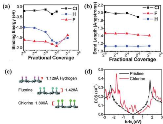
Fig. 14 (a) Binding energies and (b) bond lengths of the C–X bond (X = Cl, H, F) as functions of coverage, based on ab initio simulations. (c) Atomic structures and bond lengths of C–X. (d) Calculated DOS of graphene with a 1/30 coverage of Cl atoms in comparison with that of pristine graphene as a function of energy E - E_F , where E_F is the Fermi energy. Adapted with permission from ref. 111. Copyright (2011) American Chemical Society.
