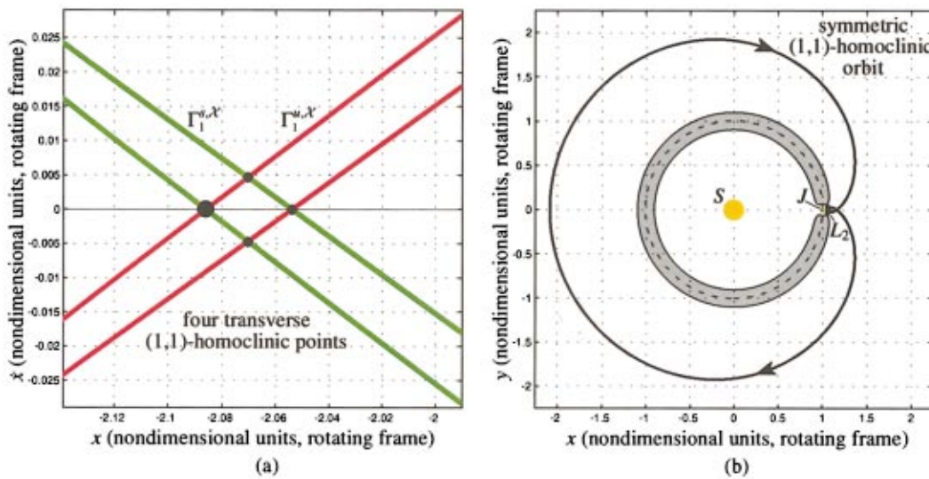
FIG. 19. (Color) (a) A group of four transverse (1,1)-homoclinic points. (b) The symmetric (1,1)-homoclinic orbit corresponding to the left \dot{x}=0 (1,1)-homoclinic point [the large black dot in (a)].
