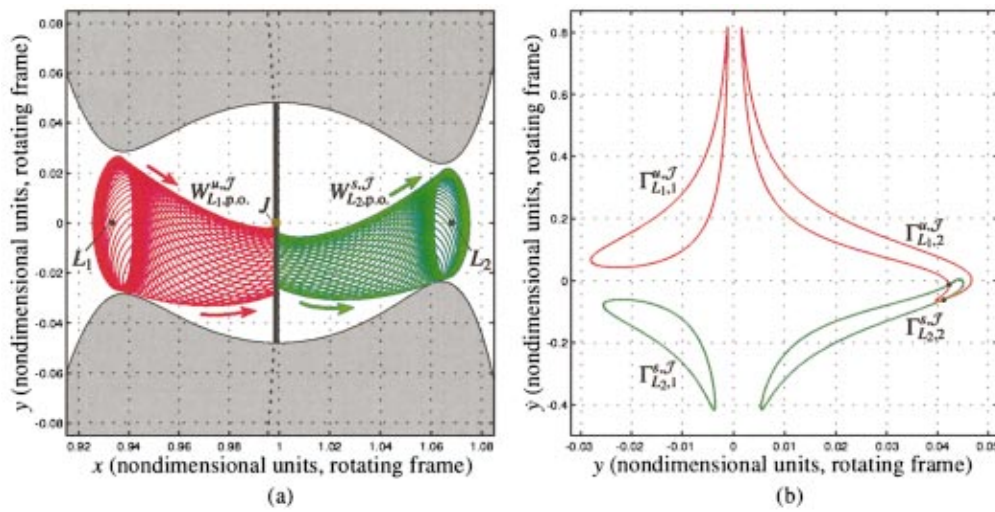
FIG. 22. (Color) (a) The projection of invariant manifolds W_{L_1,p.o.}^{u,J} and W_{L_2,p.o.}^{s,J} in the region J of the position space. (b) The first two Poincaré cuts of the invariant manifolds with the plane x=1-\mu .
