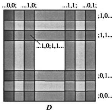
FIG. 30. The invariant set \Lambda_h of the horseshoe map h .
