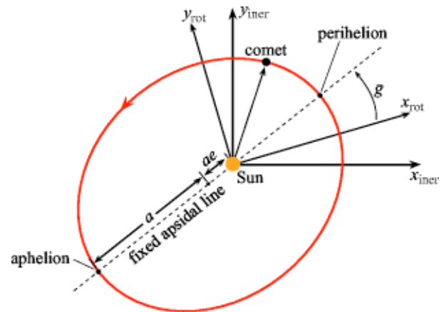
FIG. 38. (Color online) Geometry of the Delaunay variables. Elliptical orbits in the fixed (inertial) and rotating frames.
