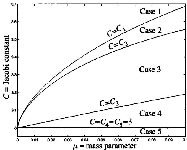
FIG. 11. The partition of the (\mu, C) -plane into five types of Hill's regions.
