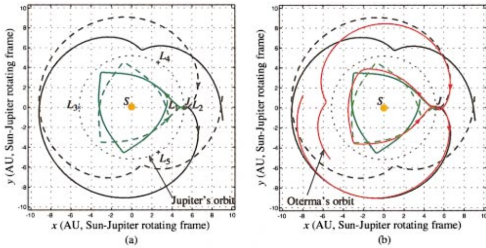
FIG. 1. (Color) (a) Stable (dashed curves) and unstable (solid curves) manifolds of L_1 and L_2 projected to position space in the Sun–Jupiter rotating frame. The L_1 manifolds are green, while the L_2 manifolds are black. (b) The orbit of comet Oterma (AD 1915–1980) in the Sun–Jupiter barycentered rotating frame (red) follows closely the invariant manifolds of L_1 and L_2 . Distances are in Astronomical Units (AU).
