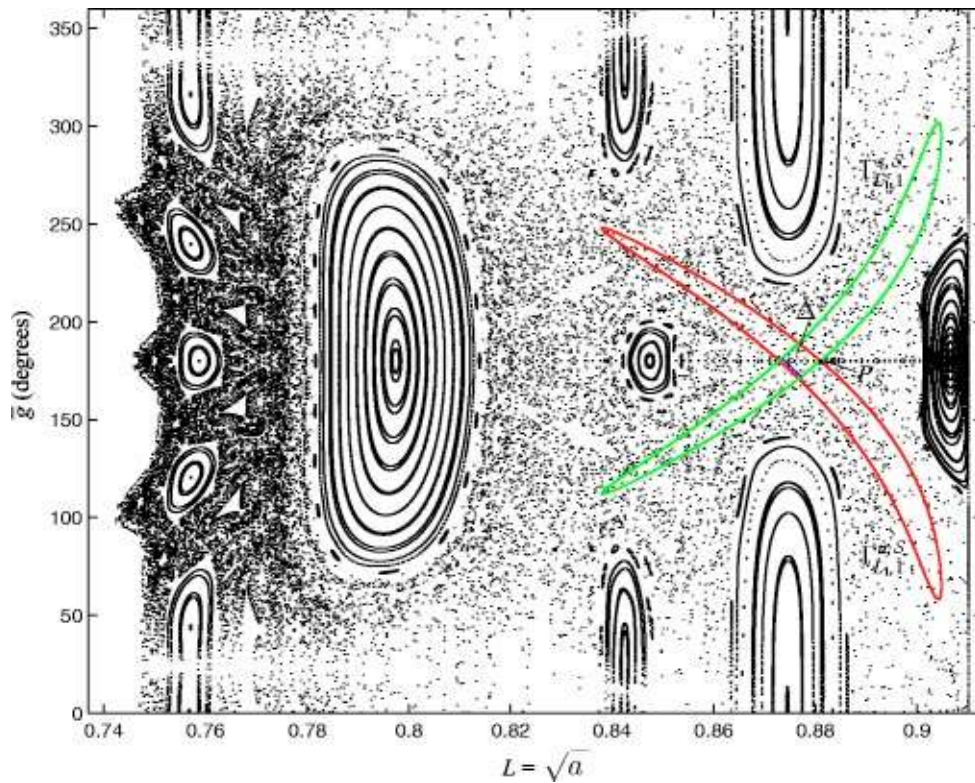
FIG. 39. (Color online) The interior region U_1 Poincaré section showing the first cuts of the stable ( \Gamma_{L_1,1}^{s,S} ) and unstable ( \Gamma_{L_1,1}^{u,S} ) manifolds of an L_1 Lyapunov orbit. Notice their intersection at the 3:2 resonance. The background points reveal the mixed phase space of stable periodic and quasiperiodic tori “islands” embedded in a bounded chaotic “sea.”
