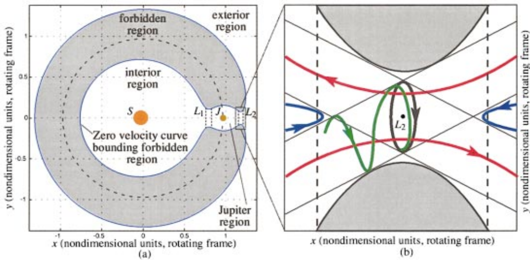
FIG. 5. (Color) (a) Hill’s region (schematic, the region in white), which contains a ‘neck’ about L_1 and L_2 . (b) The flow in the region near L_2 , showing a periodic orbit (black ellipse), a typical asymptotic orbit (green), two transit orbits (red), and two nontransit orbits (blue). A similar figure holds for the region around L_1 .
