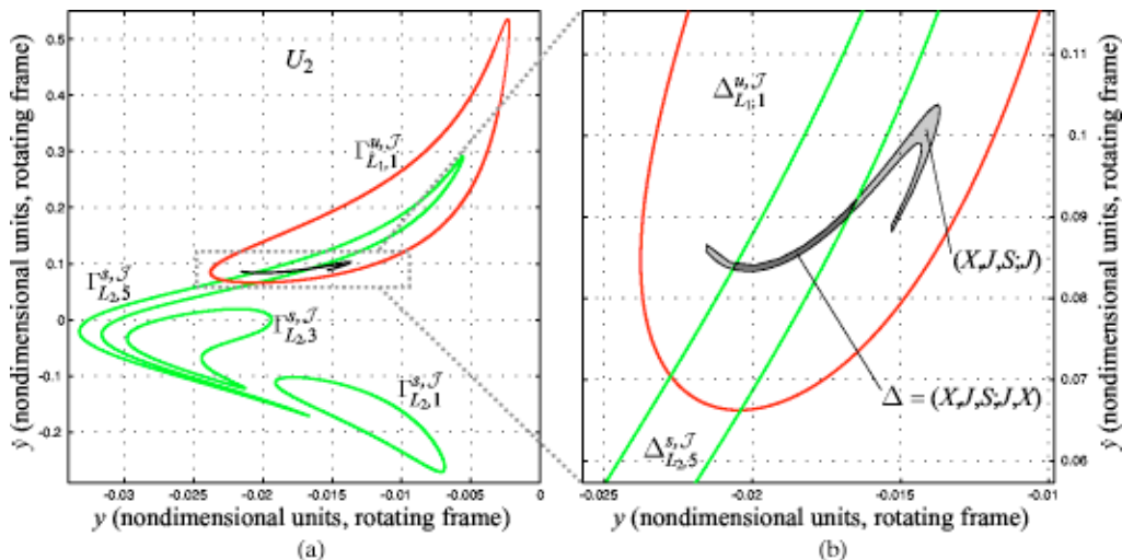
FIG. 35. (Color online) (a) Taking the (X;J;S;J) region of the U_1 Poincaré section (see Fig. 34), we evolve it until it intersects the U_2 Poincaré section ( x=1-\mu, y<0 ) in the Jupiter region (lightly shaded). Part (b) shows a close-up of the intersection of the (X;J;S;J) region with the interior \Delta_{L_{2,5}}^{S,J} of \Gamma_{L_{2,5}}^{S,J} , the fifth stable manifold cut of the L_2 Lyapunov orbit. Note the region labeled (X;J;S;J;X) , which will return to the exterior region. This region contains orbits with the desired finite itinerary.
