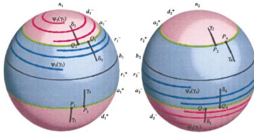
FIG. 8. (Color) Spiraling of the images of arcs \gamma_i .
