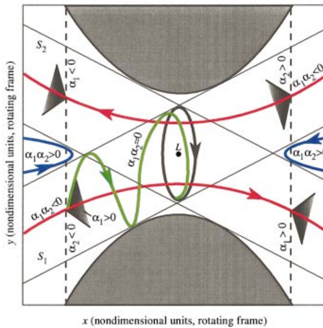
FIG. 9. (Color) The flow in the equilibrium region R of position space. Shown are the periodic orbit (black ellipse), a typical asymptotic orbit (green), two transit orbits (red), and two nontransit orbits (blue).
