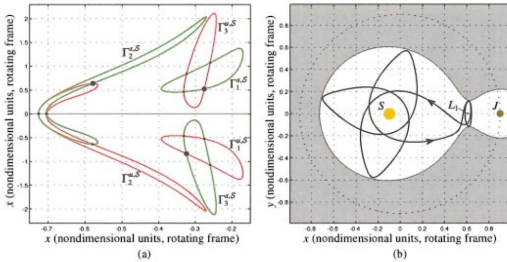
FIG. 21. (Color) (a) The first three Poincaré cuts of the unstable ( W_{L_1, p.o.}^{u,S} ) and stable ( W_{L_1, p.o.}^{s,S} ) manifolds with the plane y=0 . (b) A nonsymmetric (1,3)-homoclinic orbit in the interior region [corresponding to the large dot in (a)].
