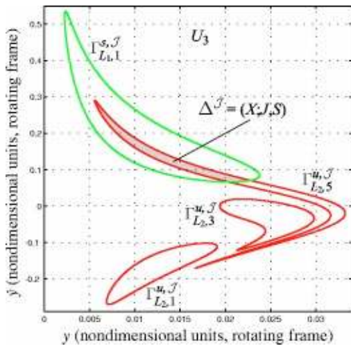
FIG. 33. (Color online) The first few transversal cuts of the L_1 (stable) and L_2 (unstable) Lyapunov orbit manifolds on the U_3 section in the Jupiter region. Notice the intersection region, in which all orbits have the central block itinerary (X;J,S) .
