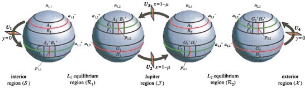
FIG. 25. (Color) The strips near the asymptotic sets on the spheres n_{1,1} , n_{1,2} , n_{2,1} , n_{2,2} .
