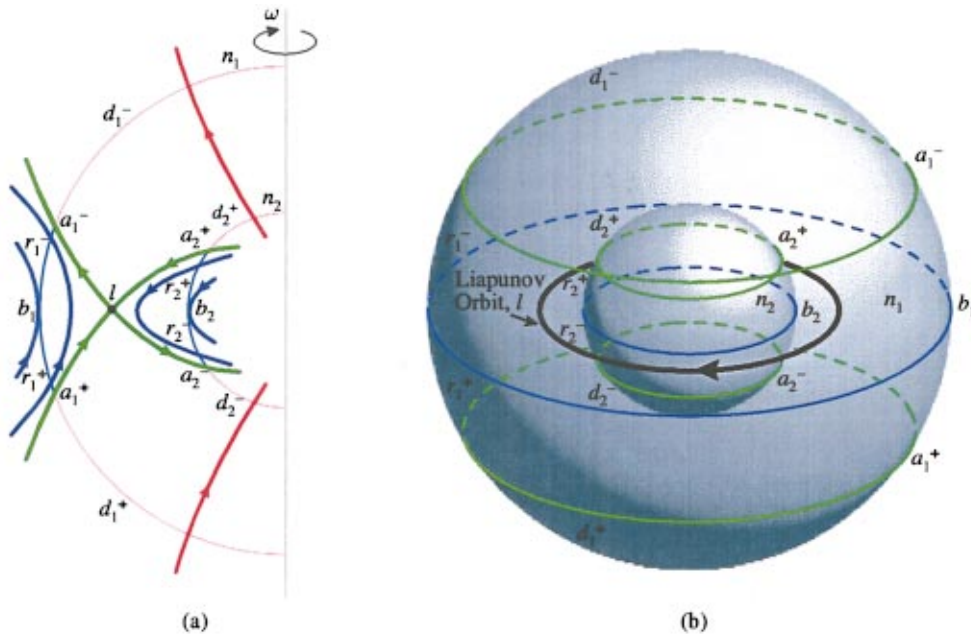
FIG. 7. (Color) (a) The cross-section of the flow in the \mathcal{R} region of the energy surface. (b) The McGehee representation of the flow in the region \mathcal{R} .
