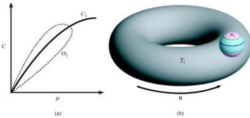
FIG. 14. (Color online) (a) Open set O_1 in the (\mu, C) -plane. (b) The invariant torus.
