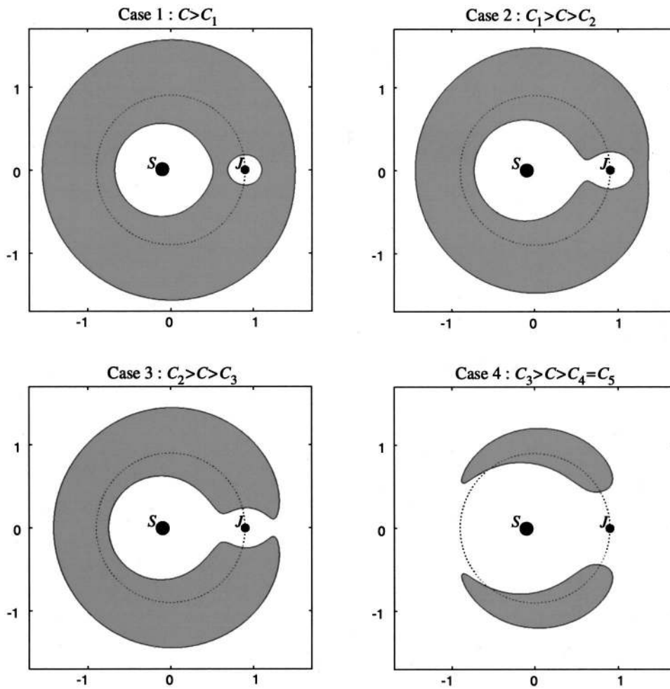
FIG. 10. Four basic configurations of the Hill's region.
