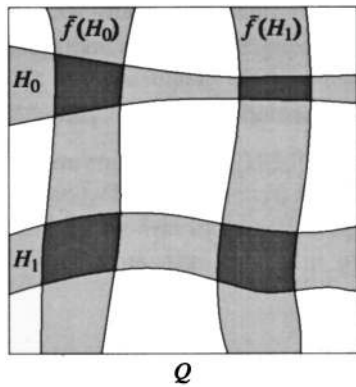
FIG. 28. Generalization of the notion of horizontal and vertical rectangles for the Conley–Moser conditions.
