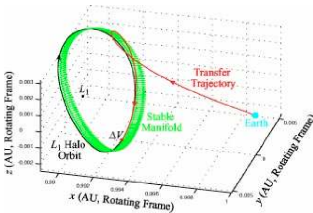
FIG. 43. (Color online) A transfer trajectory from low Earth orbit to an L_1 halo orbit. This trajectory was constructed using the stable manifold of the halo orbit. The arrows attached to the halo orbit point in the direction of the stable manifold.
