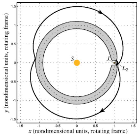
FIG. 20. (Color online) A nonsymmetric (1,1)-homoclinic point.
