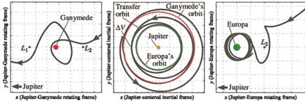
FIG. 3. (Color) The ‘Petit Grand Tour’ space mission concept for the Jovian moons. In our example, we show an orbit coming into the Jupiter system and (a) performing one loop around Ganymede (shown in the Jupiter–Ganymede rotating frame), (b) transferring from Ganymede to Europa using a single impulsive maneuver (shown in the Jupiter-centered inertial frame), and (c) getting captured by Europa (shown in the Jupiter-Europa rotating frame).
