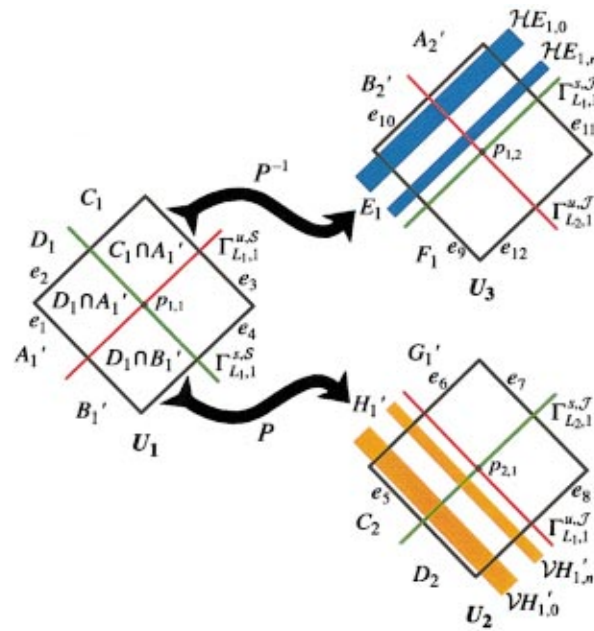
FIG. 29. (Color) The topological squares and the images of some rectangles. We show schematically only two strips although there is an infinite number.
