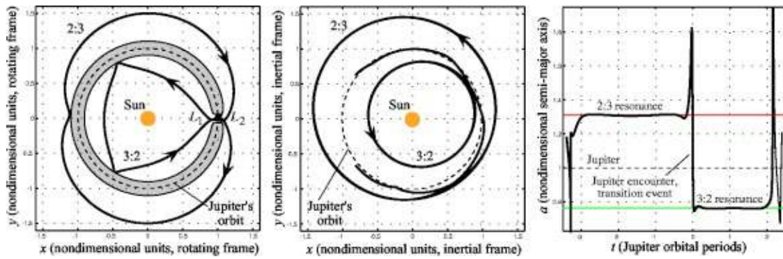
FIG. 37. (Color online) (a) The orbit \mathcal{O}' , with itinerary (J, X, J, S, J) , in the rotating frame. (b) The orbit \mathcal{O}' in the heliocentric inertial frame. (c) Plot of a vs t for the orbit \mathcal{O}' . Important mean motion resonances 3:2 and 2:3 are also shown for comparison.
