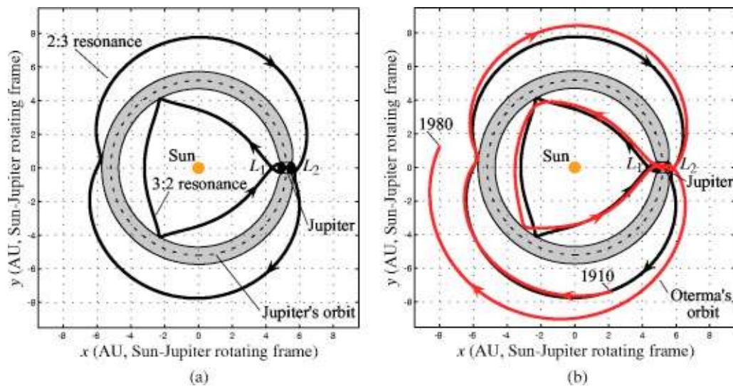
FIG. 32. (Color online) (a) The homoclinic-heteroclinic chain corresponding to the Jupiter comet Oterma . (b) The actual orbit of Oterma (AD 1910–1980) overlaying the chain.
