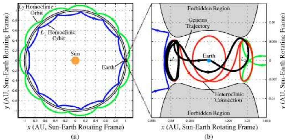
FIG. 42. (Color online) (a) A homoclinic-heteroclinic chain on the Genesis Discovery Mission trajectory's energy surface. (b) Close-up of the chain in Earth's vicinity. The actual Genesis Discovery Mission trajectory is shown in black overlaying the chain, and in particular, the heteroclinic connection from L_1 to L_2 .
