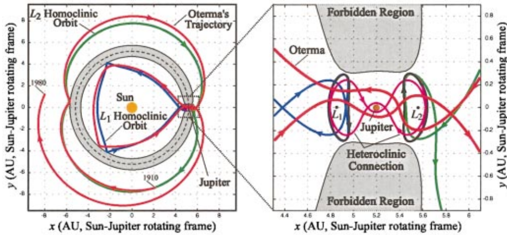
FIG. 2. (Color) A dynamical channel (homoclinic–heteroclinic chain) corresponding to the Jupiter comet Oterma . The periodic orbits about L_1 and L_2 are black. Their homoclinic orbits are blue and green. The heteroclinic connection between them is magenta. The actual orbit of Oterma (AD 1910–1980) is shown in red overlaying the chain. Distances are in Astronomical Units (AU).
