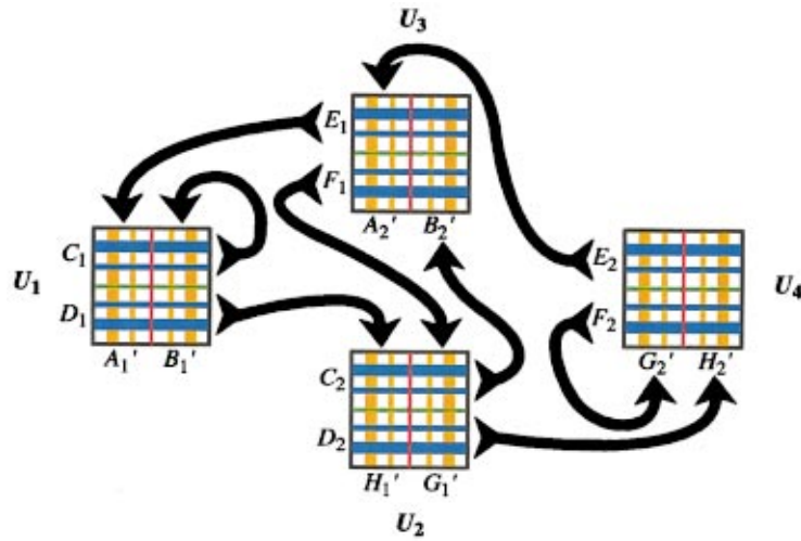
FIG. 26. (Color) The families of horizontal strips (blue) and their images (orange) under P .
