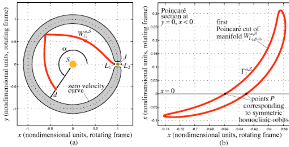
FIG. 16. (Color online) (a) Projection of the interior branch of the manifold W_{L_1}^u on the position space. (b) First intersection (Poincaré ‘‘cut’’) \Gamma_1^{u,S} of the interior branch of W_{L_1,p.o.}^u with the plane y=0 in the region x<0 .
