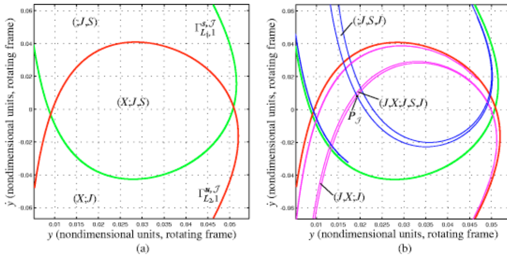
FIG. 41. (Color online) The Jupiter region U_3 Poincaré section showing the image of \Delta^X (the 2:3 resonance portion) and the pre-image of \Delta^S (the 3:2 resonance). Notice their intersections, the largest of which is labeled (J,X;J,S,J) , corresponding to the itinerary of this group of orbits.
