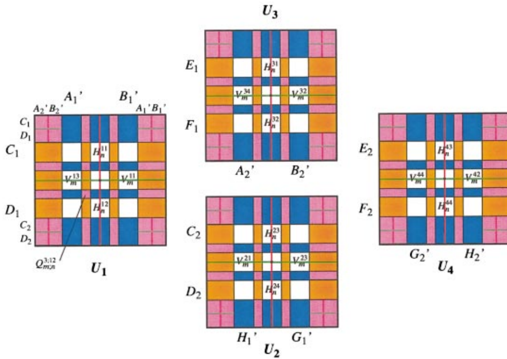
FIG. 31. (Color) The invariant set \Lambda of the Poincaré map P .
