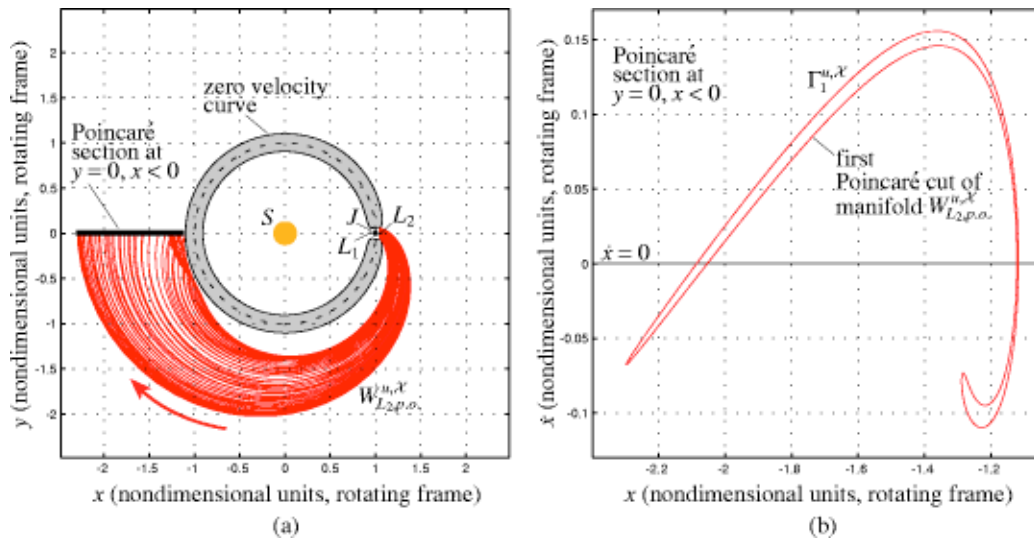
FIG. 18. (Color online) (a) The position space projection of the unstable manifold “tube” W_{L2,p.o.}^{u,\mathcal{X}} until the first intersection with the Poincaré section at y=0, x<0 . (b) The first Poincaré cut \Gamma_1^{u,\mathcal{X}} of the manifold W_{L2,p.o.}^{u,\mathcal{X}} on the plane y=0, x<0 .
