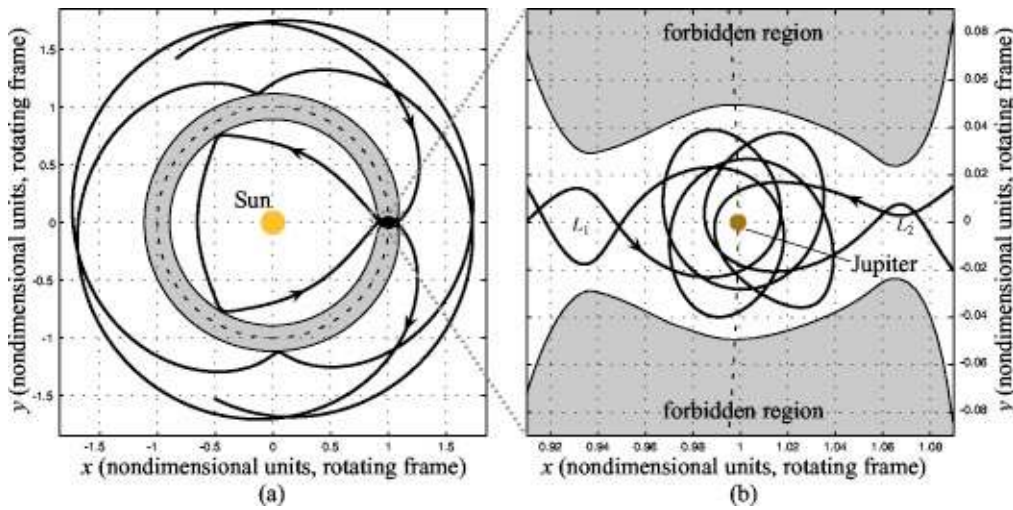
FIG. 36. (Color online) (a) An orbit with the itinerary (\dots, X, J, S, J, X, \dots) computed using an initial condition inside the \Delta region of the U_2 section (see Fig. 35). (b) A close-up of this orbit in the Jupiter region.
