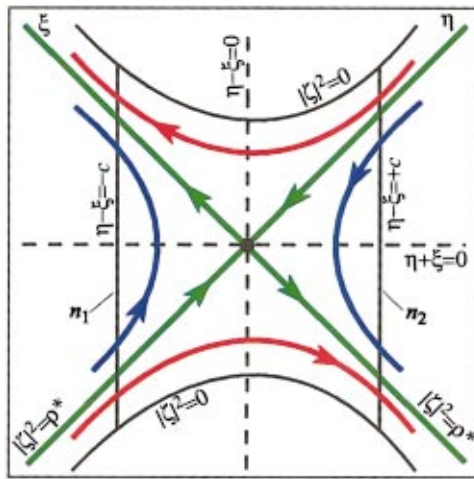
FIG. 6. (Color) The projection onto the (\eta, \xi) -plane of orbits near the equilibrium point (note, axes tilted 45^\circ ). Shown are the periodic orbit (black dot at the center), the asymptotic orbits (green), two transit orbits (red), and two non-transit orbits (blue).
