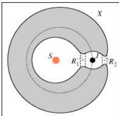
FIG. 13. (Color online) Division of Hill's region into five sets.
