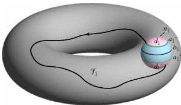
FIG. 15. (Color online) The existence of orbits homoclinic to the Lyapunov orbit.
