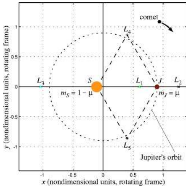
FIG. 4. (Color online) Equilibrium points of the planar circular restricted three-body problem as viewed, not in any inertial frame, but in the rotating frame, where the Sun and Jupiter are at fixed positions along the x -axis.
