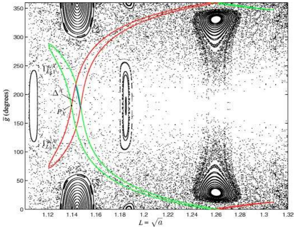
FIG. 40. (Color online) The exterior region U_4 Poincaré section showing the first cuts of the stable ( \Gamma_{L_2,1}^{s,\chi} ) and unstable ( \Gamma_{L_2,1}^{u,\chi} ) manifolds of an L_2 Lyapunov orbit. Notice their intersections at the 2:3 and 1:2 resonances. The background points reveal a mixed phase space similar to that of Fig. 39.
