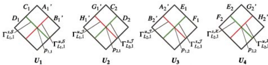
FIG. 27. (Color) The domain U = U_1 \cup U_2 \cup U_3 \cup U_4 of the Poincaré map P .
