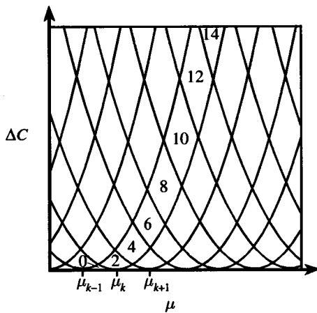
FIG. 17. Partition of the (\mu, \Delta C) -plane according to the number of symmetric (1,1)-homoclinic points found in the first intersection of W_{L_1, p.o.}^{u,s} with the plane y=0, x<0 .
