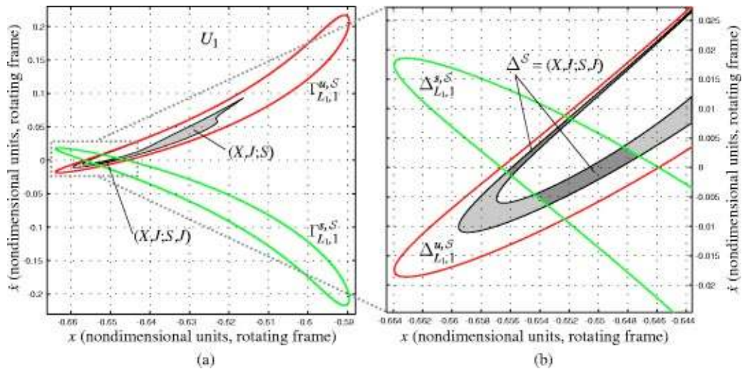
FIG. 34. (Color online) (a) Taking the (X;J;S) region of the U_3 Poincaré section (see Fig. 33), we evolve it until it intersects the U_1 Poincaré section in the interior region (lightly shaded). (b) A close-up of the intersection of the (X;J;S) region with the interior \Delta^{S,S} of \Gamma_{L_{1,1}}^{S,S} , the first stable manifold cut of the L_1 Lyapunov orbit. Note the regions labeled (X;J;S;J) , which will return to the Jupiter region.
