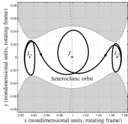
FIG. 23. (Color online) The existence of a transversal (2, 2) -heteroclinic orbit in the J region.
