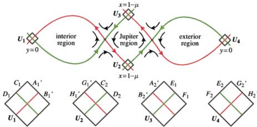
FIG. 24. (Color) The construction of a suitable Poincaré map.
