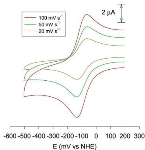
Fig. 7 Cyclic voltammety of [\text{Fe}(\text{PSMC})(\text{PCSMC})] at 20, 50 and 100 \text{mV s}^{-1} sweep rate: MeCN– \text{H}_2\text{O} (7 : 3) with 0.1 M \text{Et}_4\text{NClO}_4 supporting electrolyte.
