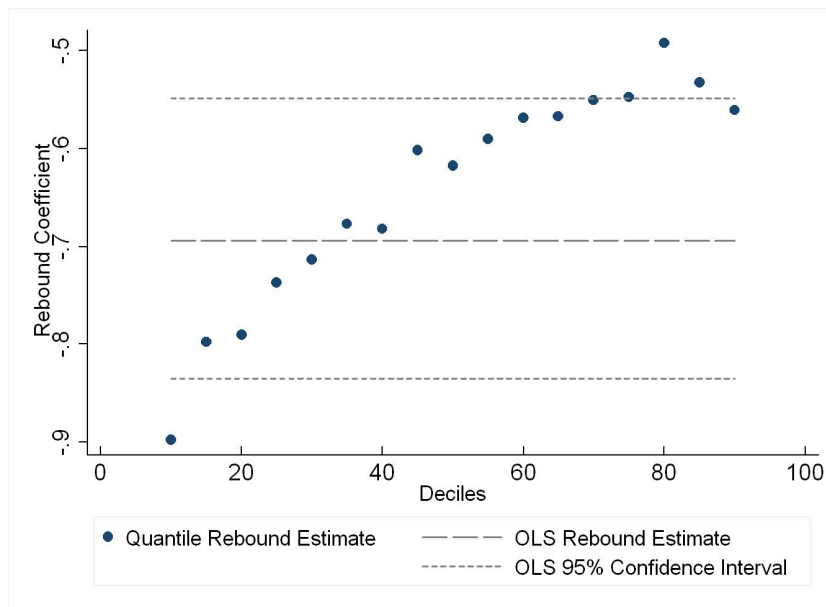
Figure 1: Comparison of the OLS and Quantile Regression Results for the Rebound Effect according to Definition 4.
