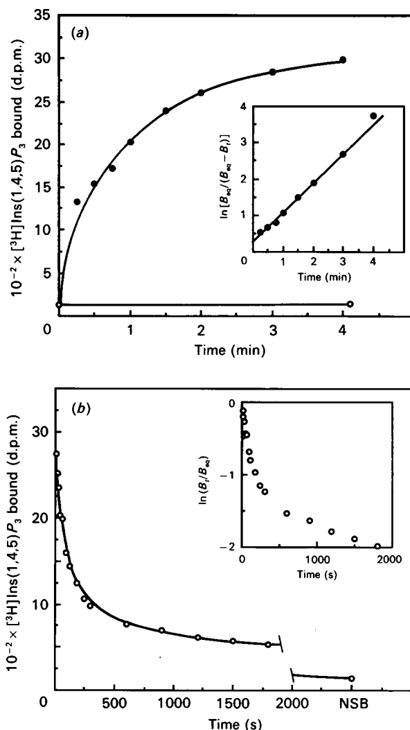
Fig. 3. Association (a) and dissociation (b) rates for [^3\text{H}]\text{Ins}(1,4,5)\text{P}_3 binding to adrenal-cortex membranes
