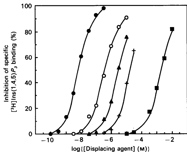
Fig. 2. Specificity of [^3\text{H}]\text{Ins}(1,4,5)\text{P}_3 binding to adrenal-cortex membranes
