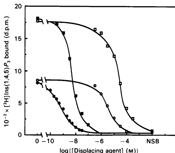
Fig. 4. Comparison of displacement of [^3\text{H}]\text{Ins}(1,4,5)\text{P}_3 at 0.15 nM and 1.5 nM by unlabelled \text{Ins}(1,4,5)\text{P}_3 in adrenal-cortex membranes
