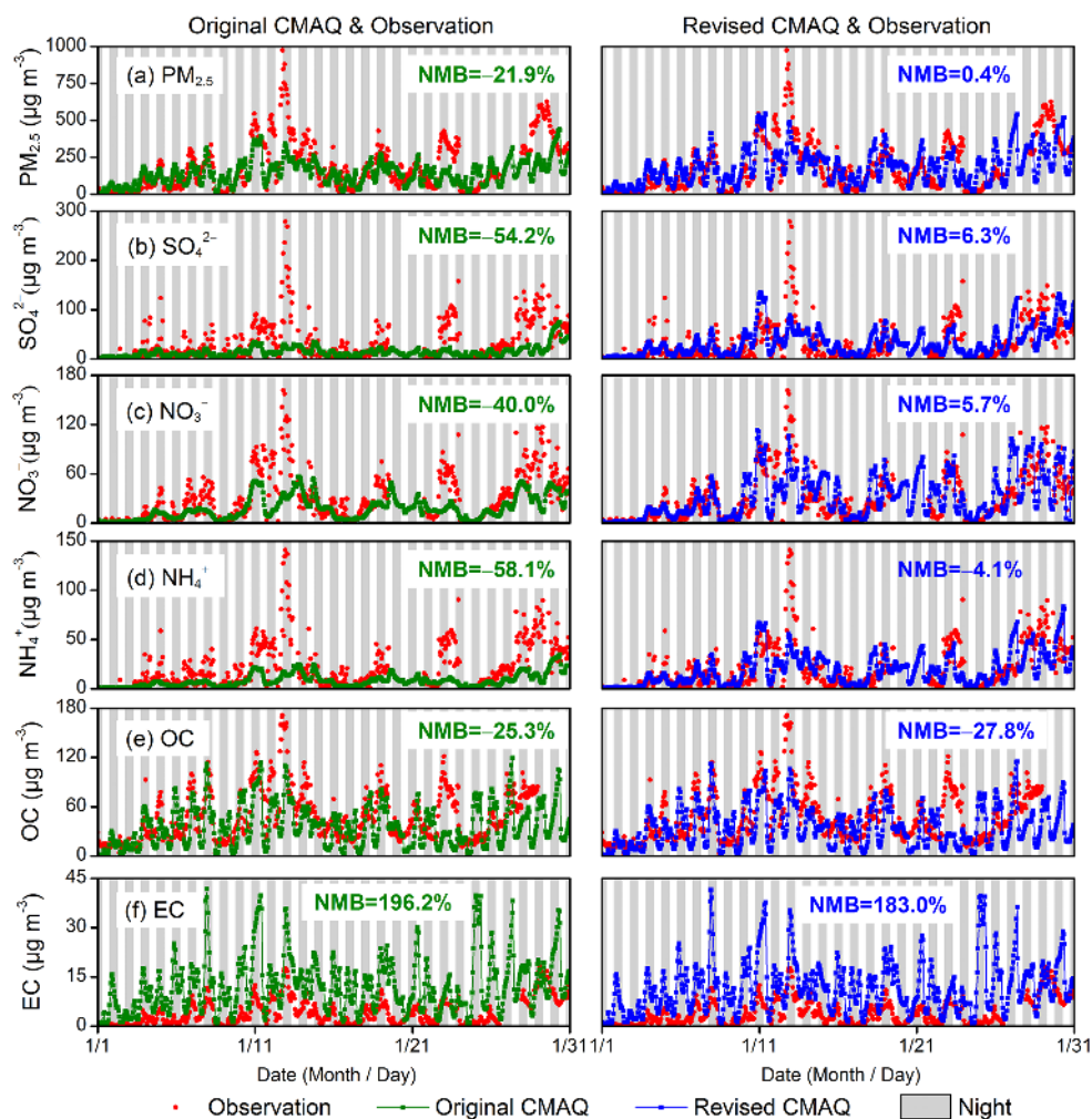
Figure 4. Observed and simulated hourly aerosol compositions from the original and revised CMAQ at the THU site: (a) PM 2.5 ; (b) SO 4 2- ; (c) NO 3 - ; (d) NH 4 + ; (e) OC; (f) EC.
