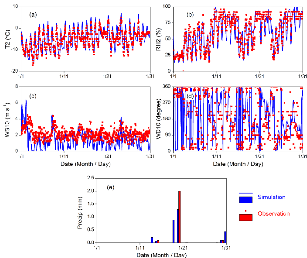
Figure 3. Observed and simulated meteorological variables at THU site: (a) hourly T2; (b) hourly RH2; (c) hourly WS10; (d) hourly WD10; (e) daily Precip.
