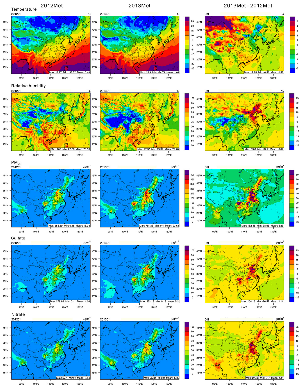
Figure 8. Spatial distributions of the monthly (January 2013) mean temperature, RH and concentrations of \text{PM}_{2.5} , sulfate and nitrate simulated by the revised CMAQ model with meteorological fields of 2012 (left) and 2013 (middle), and the differences between these two simulations (right).
