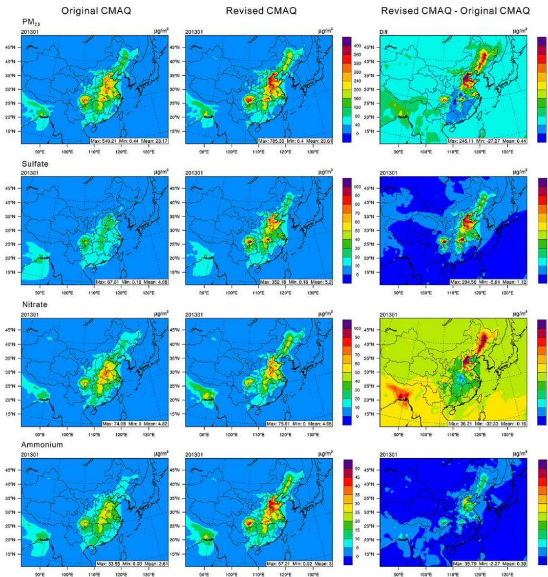
Figure 6. Spatial distributions of monthly (January 2013) mean concentrations of PM 2.5 , sulfate, nitrate and ammonium simulated by the Original CMAQ (left), Revised CMAQ (middle) and the differences between the Revised and Original CMAQ (right).
