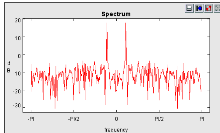
FIGURE 2.68. Still better labeled plot.
