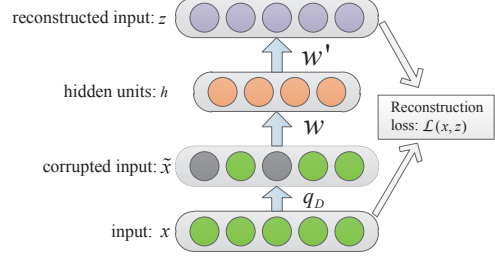
Fig. 4. Illustration of denoising autoencoder. The inputs are corrupted by a corruption map q_D , and we reconstruct the original input from this corrupted \tilde{x} . We train all the hidden layer by minimizing the reconstruction error \mathcal{L} between the uncorrupted input x and the reconstructed z .
