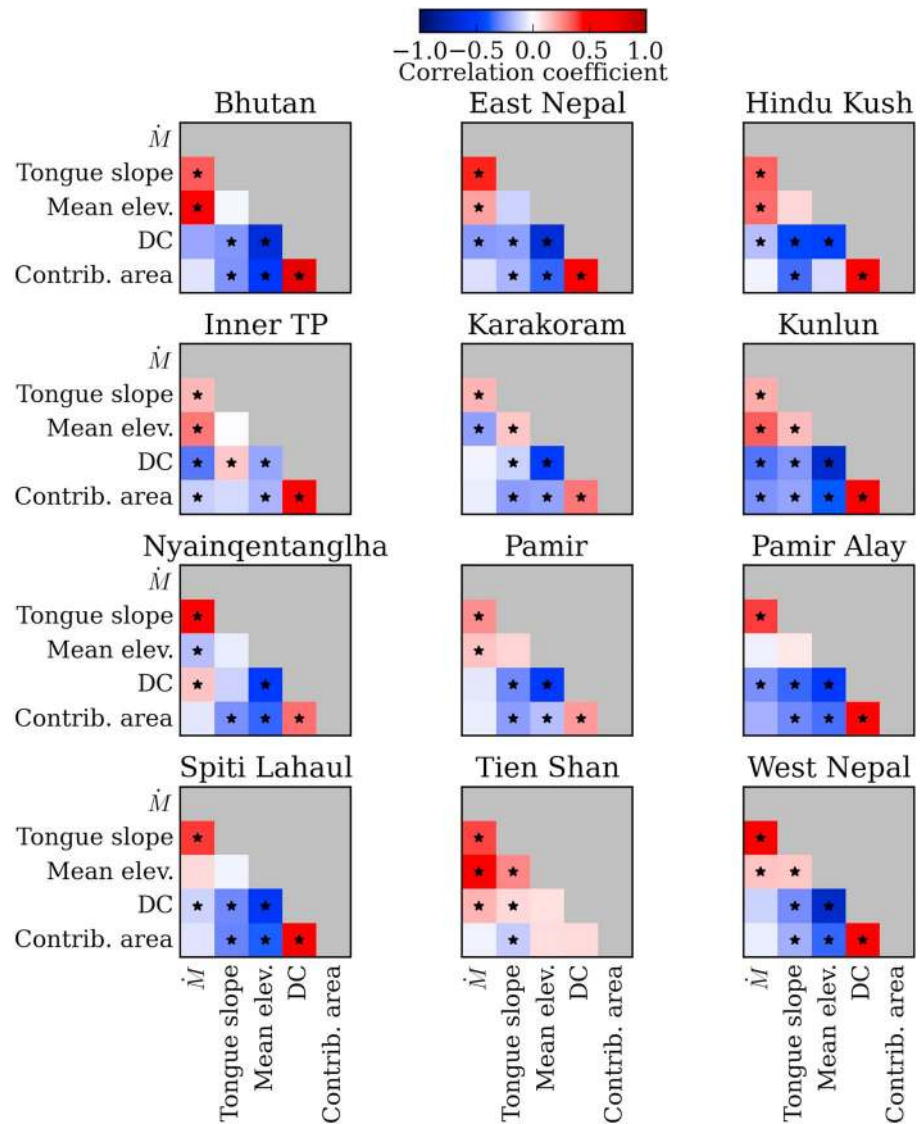
Figure 4. Pearson correlation coefficients between selected variables. The ★ denotes correlation significant at p < 0.01 . DC = debris cover; TP = Inner Tibetan Plateau.
