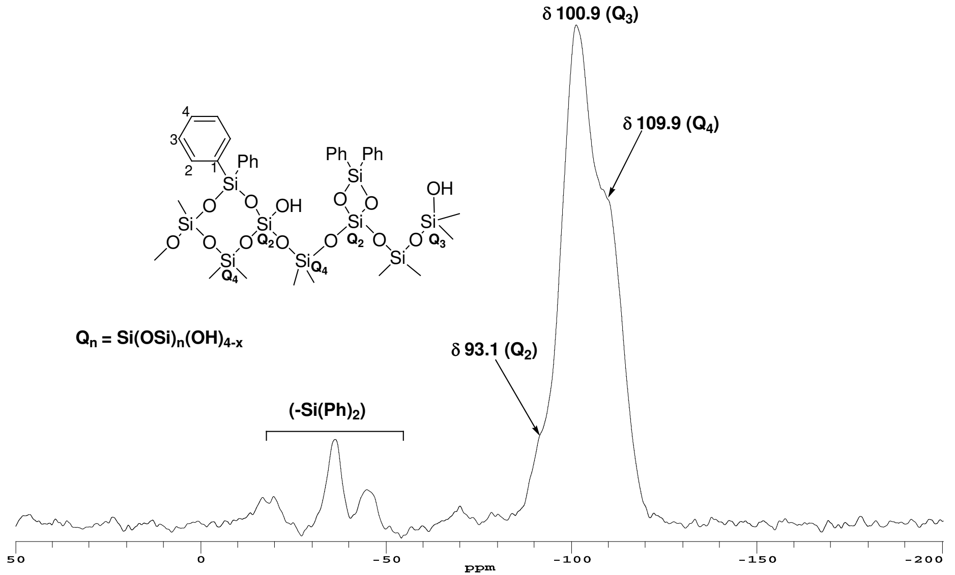
Figure 5. ^{29}\text{Si} CP/MAS NMR of Chemically Modified MCM-41
