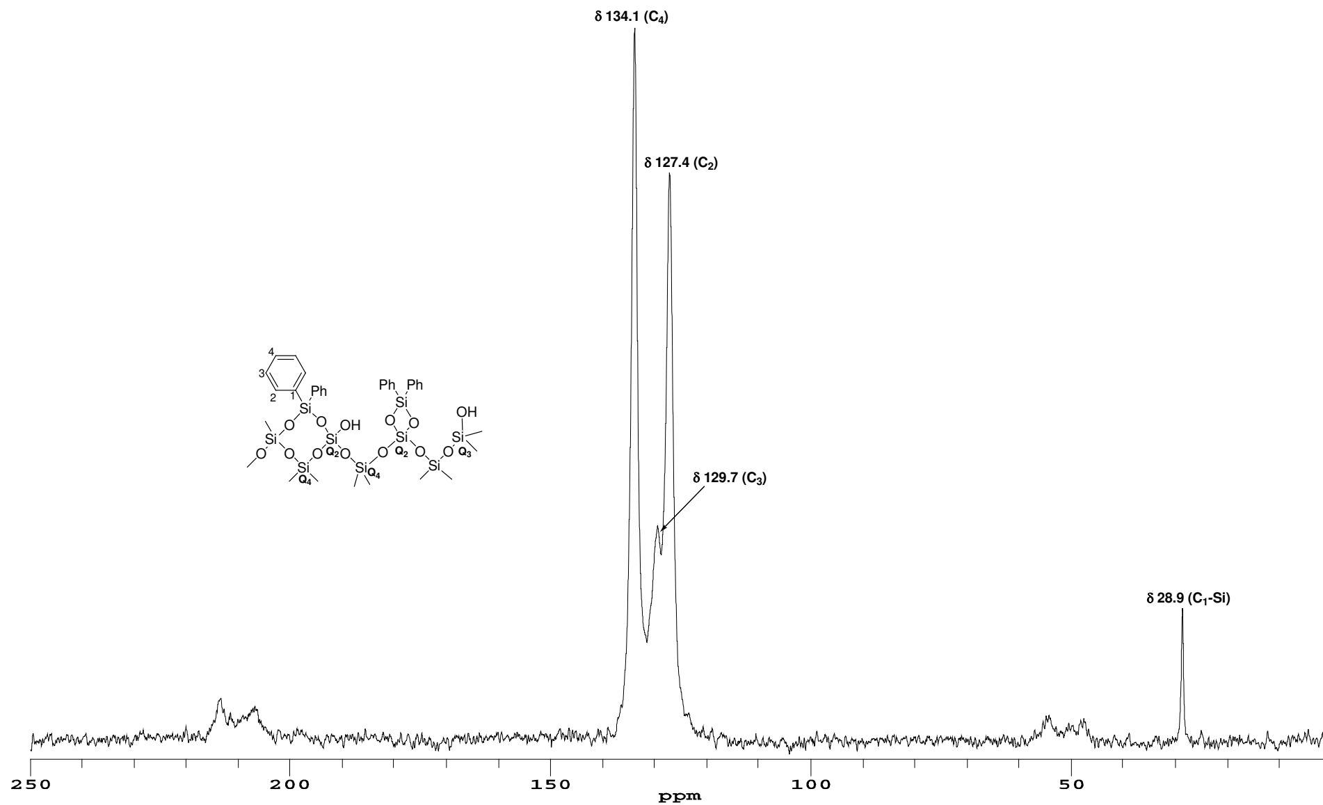
Figure 6. ^{13}\text{C}\{^1\text{H}\} CP/MAS NMR of Chemically Modified MCM-41
