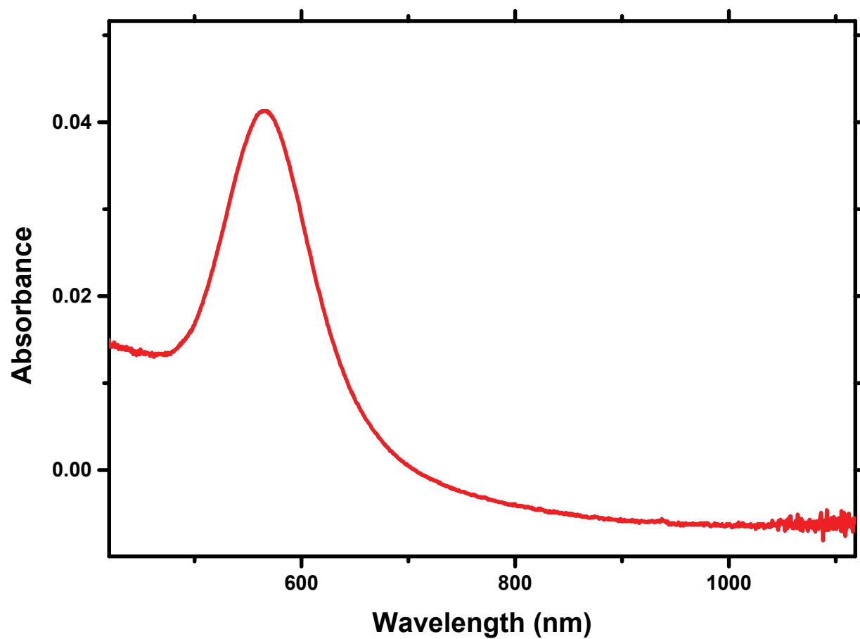
Figure SIS-2: The optical absorbance of the gold nanoparticles used in this experiment. The particles were dispersed on glass. An uncoated portion of the sample was used as the reference for the absorbance measurement.
