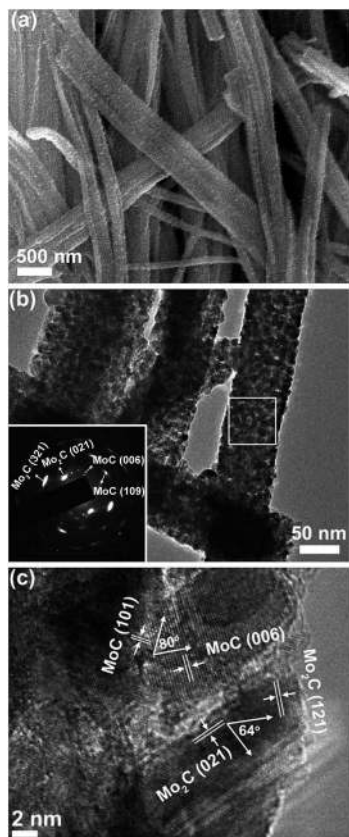
Fig. 2 (a) SEM, (b) TEM and (c) HR-TEM images of MoC–Mo 2 C-31.4 HNWs. Inset of (b) is the SAED pattern obtained on the marked area.
