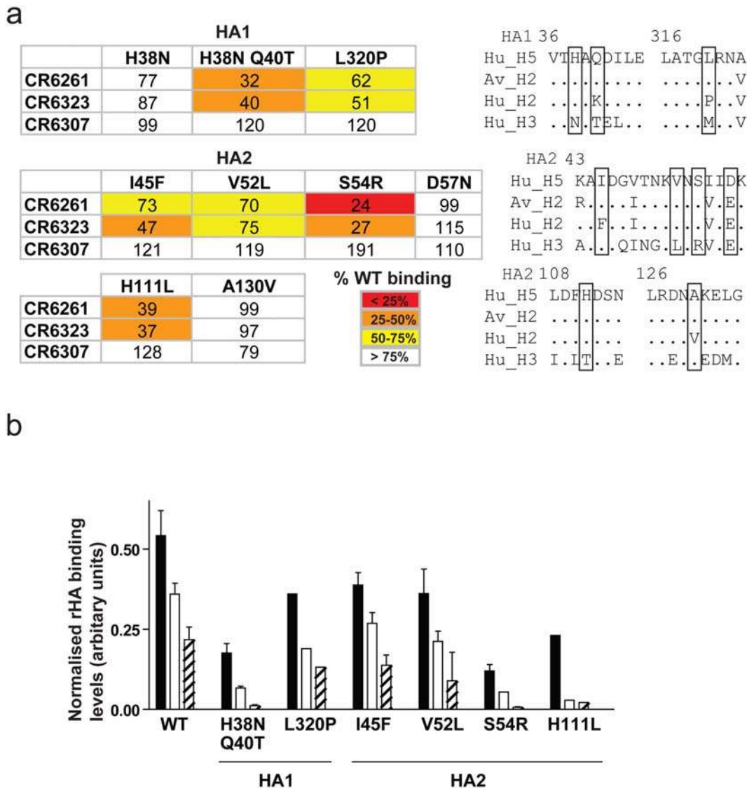
Figure 9. Binding of CR6261 to H5 HA point mutants. (a) FACS binding of IgG1 to surface expressed mutants of H5 rHA. Mean fluorescent intensity (MFI) values were normalised to NIBRG-14 antiserum reactivity to the corresponding mutant and expressed as the average percentage of wild type H5 rHA binding from two independent experiments (see key for colour code). Adjacent are sequence alignments of the corresponding region, mutated residues are boxed. (b) FACS binding activity to WT or mutant H5 rHA performed as above for CR6261 (solid bars), CR6261 with the HCDR2 mutation F54L (open bars) or F54A (striped bars). MFI was normalised as above and expressed as mean \pm s.e.m. arbitrary units from two independent experiments.
