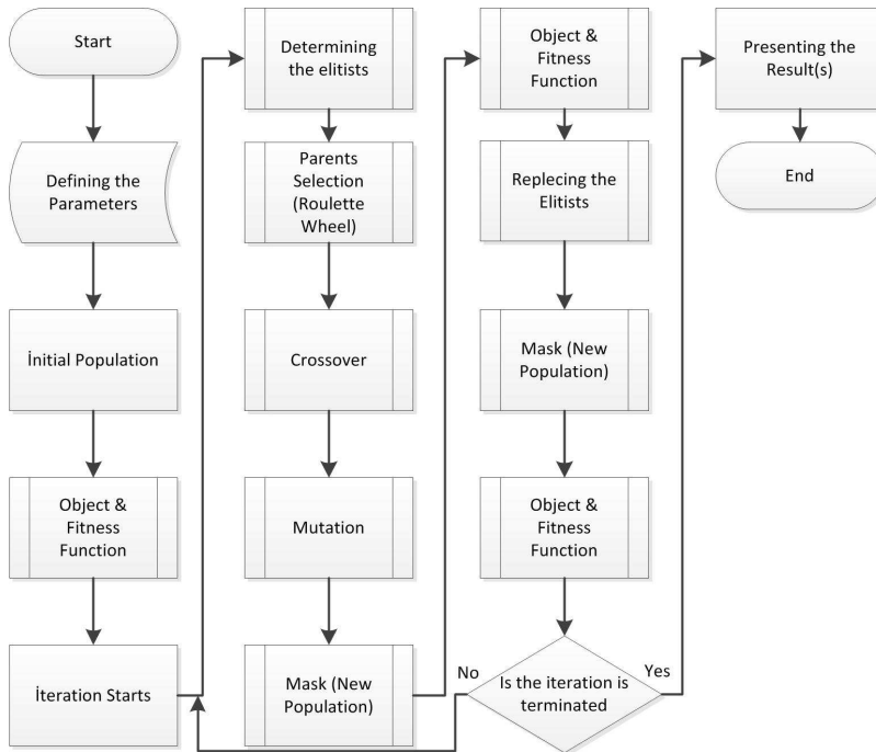
Fig. 11. The flowchart of the GA
