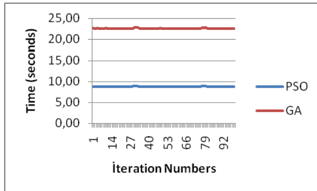
Fig. 16. The execution times of the two algorithms
