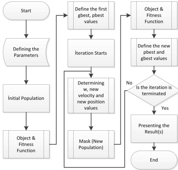
Fig. 13. The flowchart of the PSO algorithm
