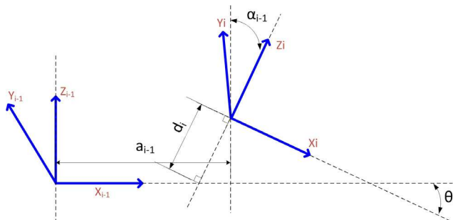
Fig. 8. DH parameters between two coordinate systems
