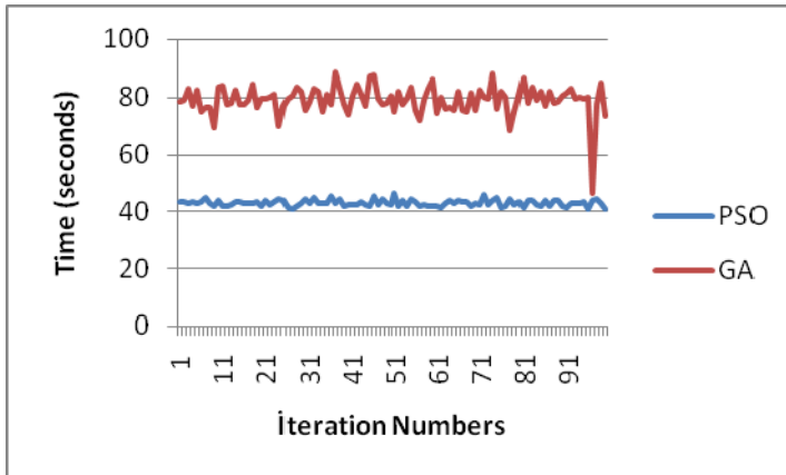
Fig. 22. The execution times of the two algorithms
