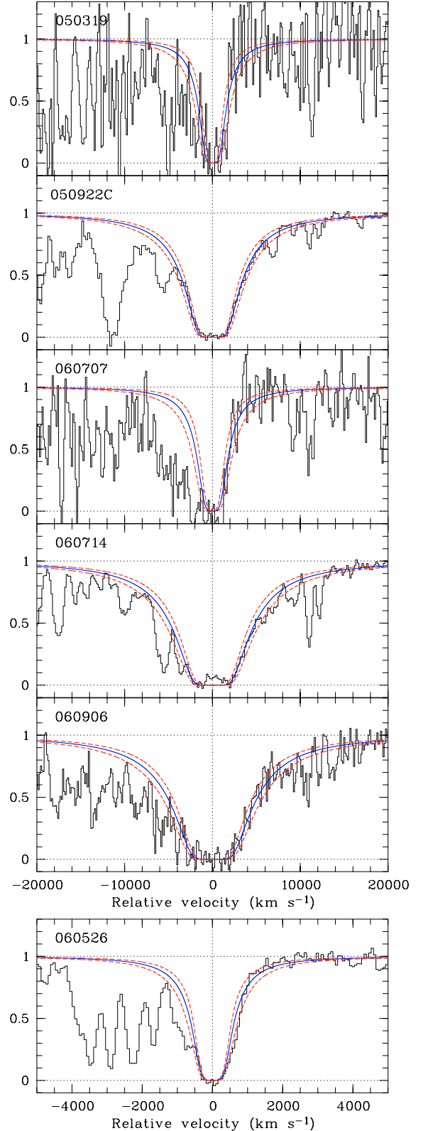
Fig. 1. The normalized OA spectra centred on the Ly \alpha absorption lines at the GRB host galaxy redshifts. A neutral hydrogen column density fit to the damped Ly \alpha line is shown with a solid line in each panel, while the 1\sigma errors are shown with dashed lines.
