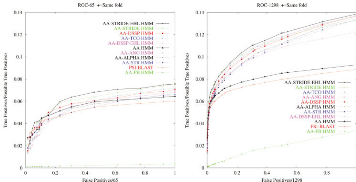
Fig. 9. Results of three-fold cross-validated fold recognition tests on our benchmark dataset (dunbrack-in-scop) shown for two-track HMMs with an amino acid primary track and STRIDE-EHL, STRIDE, DSSP, TCO, DSSP-EHL, ANG, ALPHA, STR, and PB on the secondary track, amino-acid only HMMs, and PSI-BLAST run with four iterations. (a) ROC_{65} . Number of negatives recognized fixed at 65 (0.05 false positives per query). (b) ROC_{1298} . Number of negatives recognized fixed at 1298 (1.0 false positives per query). The methods are ranked in the legends according to ROC_N score. As shown in (a), with a strict threshold of 0.05 false positives per query AA-STRIDE-EHL HMMs have the best accuracy by a small margin. With looser thresholds of 0.1 to 1.0 false positives per query, shown in (b), the accuracy of all the local structure HMMs is significantly better than that of the AA-only methods. AA-DSSP-EHL HMMs perform comparably to the other good two-track HMMs in the range below 0.5 false positives per query but are less accurate in the range above 0.5 false positives per query. The poor performance of AA-PB HMMs is an artifact of the reverse-sequence null model SAM uses to compute HMM scores. 53
