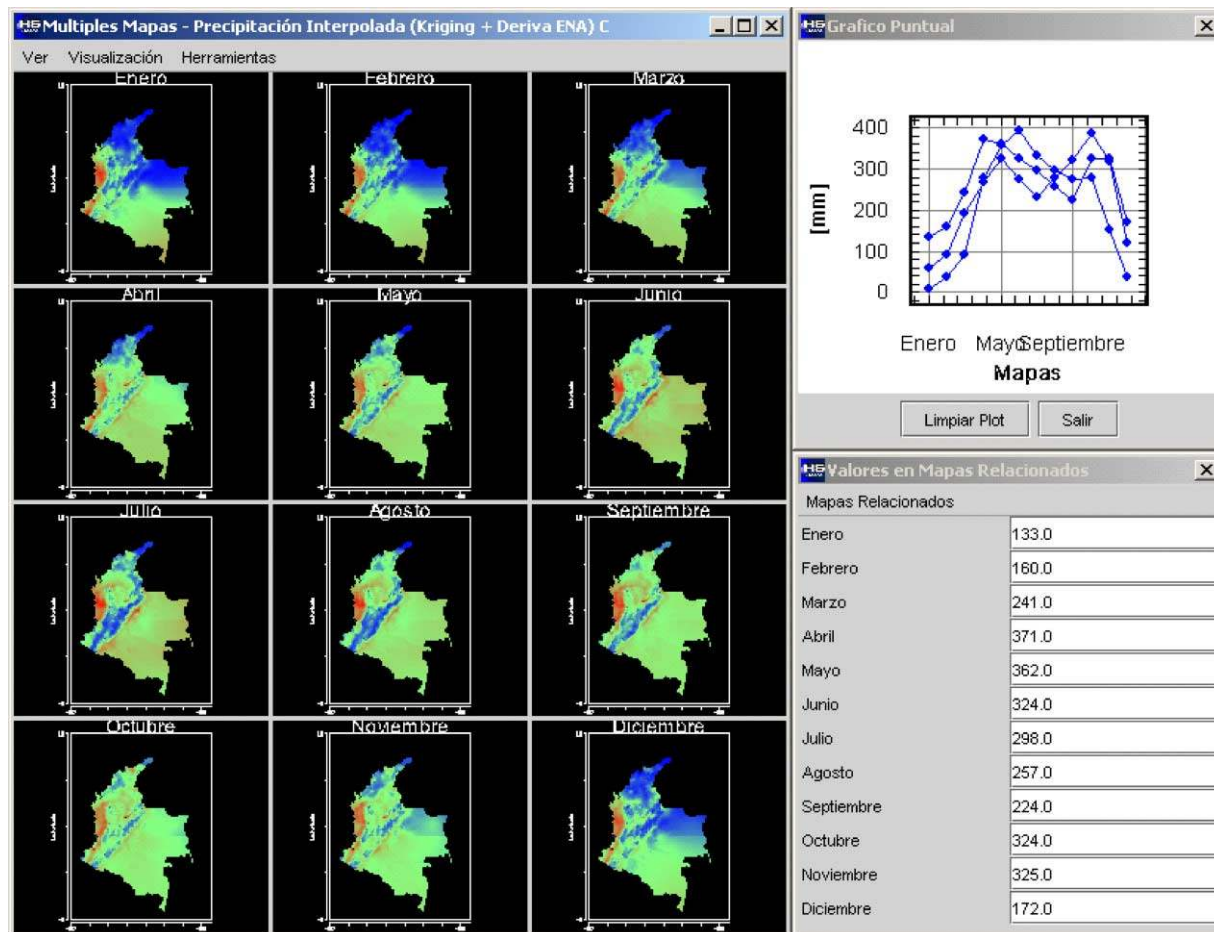
Figure 3 | HydroSIG's display of the twelve maps of average monthly precipitation over Colombia. Data on monthly precipitation at selected sites are given in the right-hand panels, both in graphical and tabular formats.
