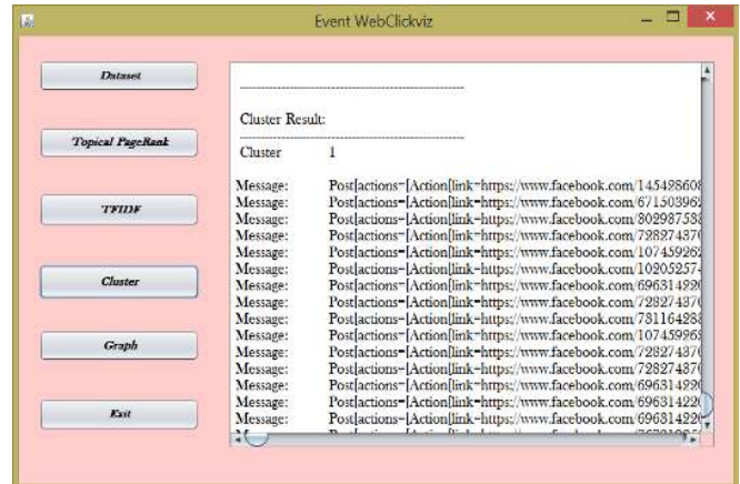
Figure.5. Clustering results
