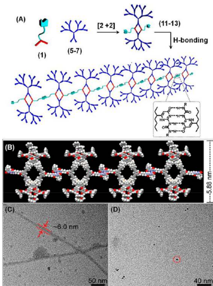
Figure 3. (A) Synthesis and formation of DSPs of UPy-functionalized rhomboids 11–13 . (B) DSP of 13 by PM6 semiempirical molecular orbital methods. TEM images of aggregates of 13 obtained from (C) \text{CH}_2\text{Cl}_2 and (D) DMSO. Adapted with permission from ref 15. Copyright 2013 American Chemical Society.
