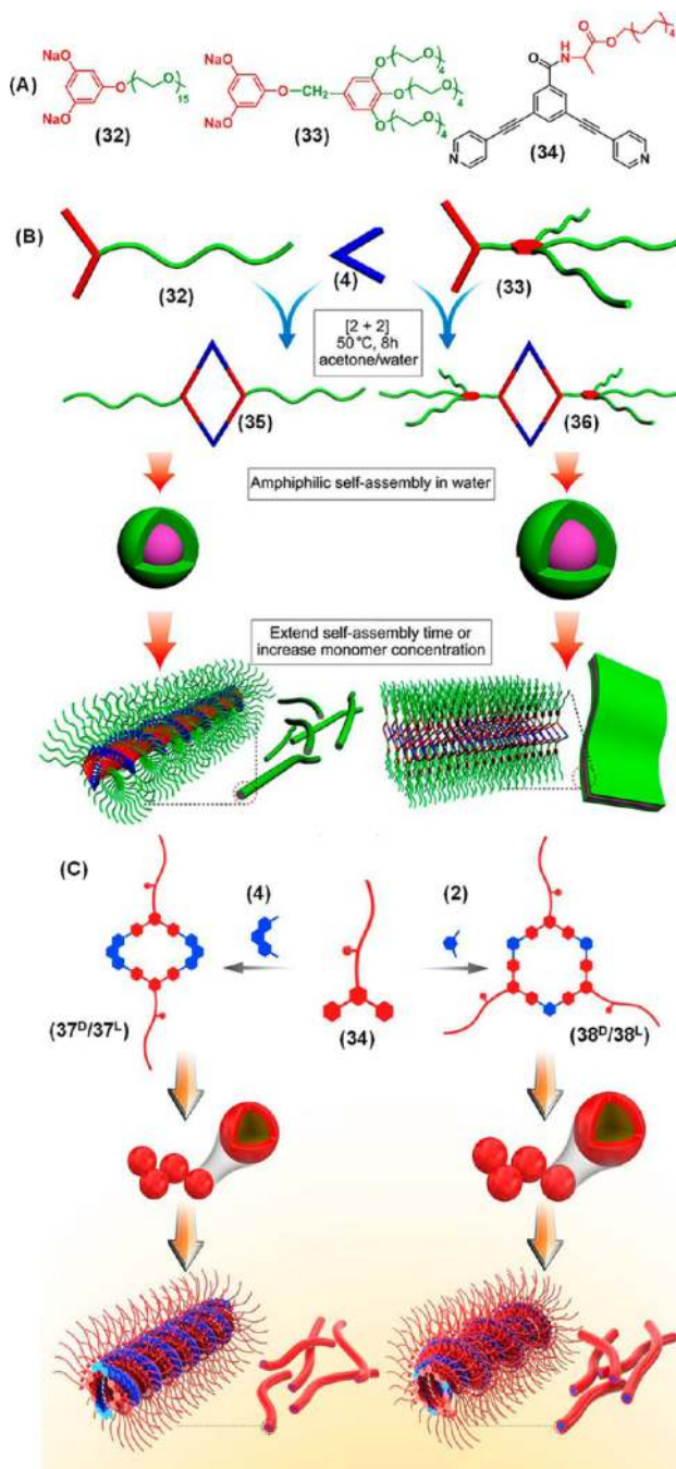
Figure 10. (A) Precursors reported by Yan et al. 30 and Sun et al. 31 for the preparation of metallacycles. Schematic illustration of the formation of various nanostructures by (B) 35 and 36 and (C) 37 D /37 L and 38 D /38 L depending upon concentration. Panel B Adapted with permission from ref 30. Copyright 2013 American Chemical Society. Panel C Adapted with permission from ref 31. Copyright 2017 American Chemical Society.
