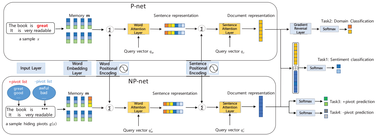
Figure 1: The framework of the HATN model.
