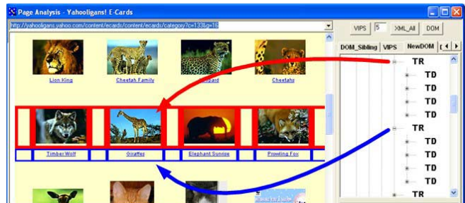
b) Partition on DOM tree (The red area and blue area are two different TR nodes)
