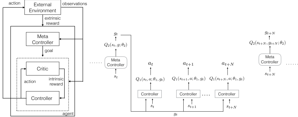
Figure 1: (Overview) The agent receives sensory observations and produces actions. Separate DQNs are used inside the meta-controller and controller . The meta-controller looks at the raw states and produces a policy over goals by estimating the action-value function Q_2(s_t, g_t; \theta_2) (to maximize expected future extrinsic reward). The controller takes in states and the current goal, and produces a policy over actions by estimating the action-value function Q_1(s_t, a_t; \theta_1, g_t) to solve the predicted goal (by maximizing expected future intrinsic reward). The internal critic provides a positive reward to the controller if and only if the goal is reached. The controller terminates either when the episode ends or when g is accomplished. The meta-controller then chooses a new g and the process repeats.
