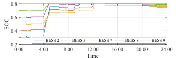
(b) L group SOC curves.
