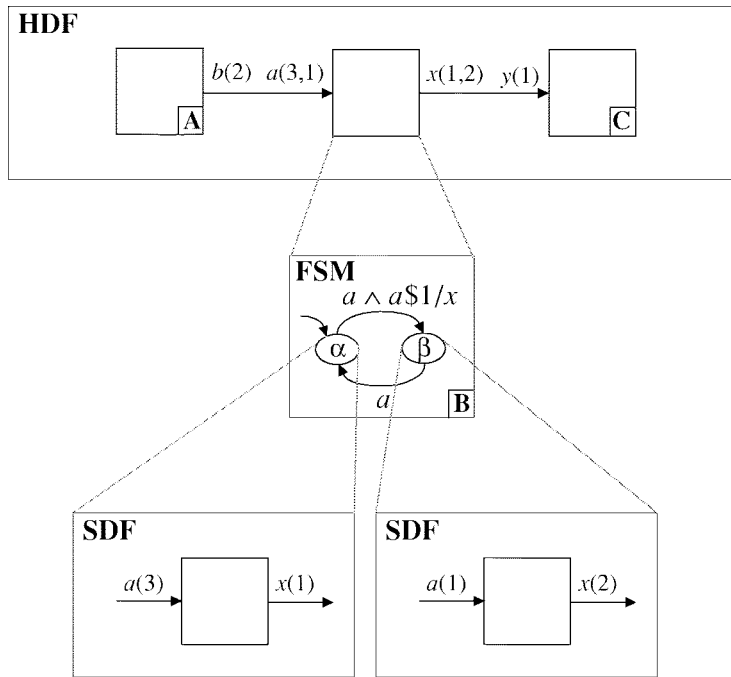
Fig. 12. An FSM with states that refine to SDF subsystems with different type signatures.
